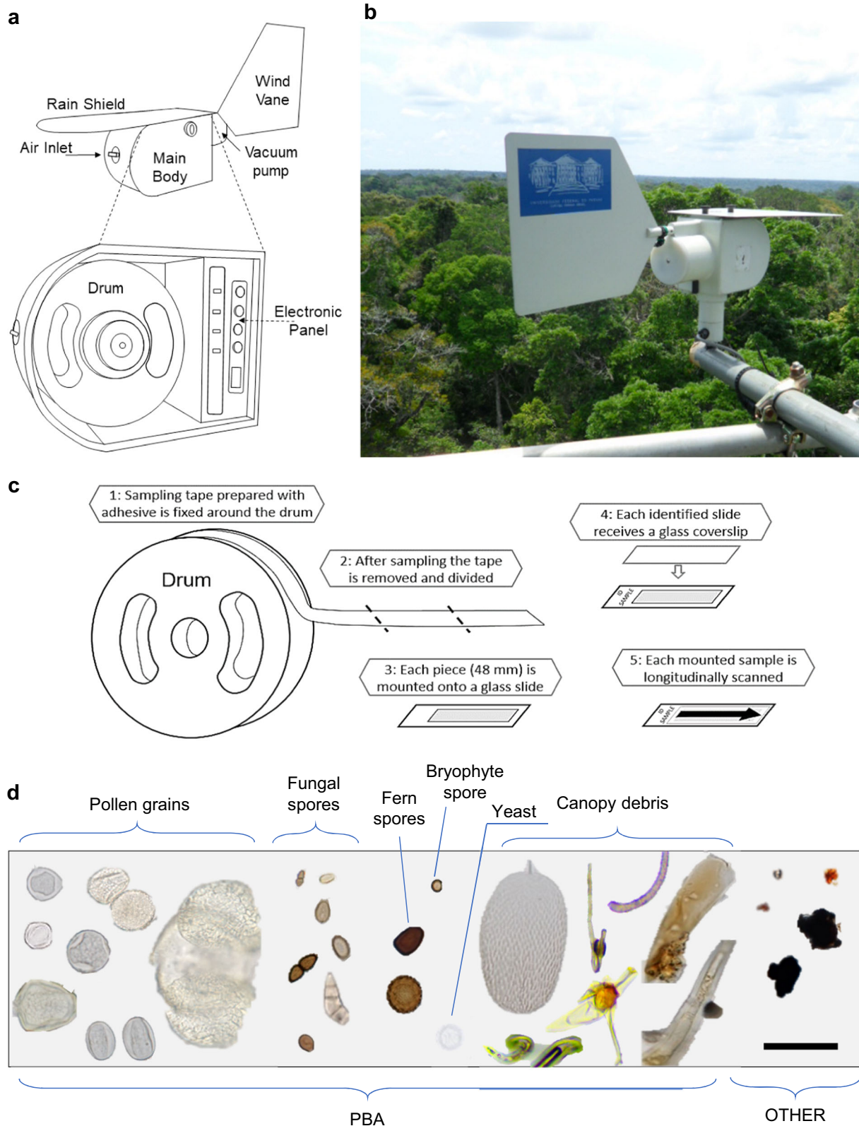
Fig. 6 Equipment and method of sampling. a Drawing scheme of the Burkard Volumetric Spore Sampler describing the parts attached to the main body, with the internal view in detail showing the rotating drum; b Picture of the sampler attached to the tower by a metallic support allowing free rotation according to the wind direction; c Scheme of the steps followed during sampling: (1) sampling tape preparation with adhesive along the entire surface and fixation on the side of the rotating drum, (2) removal of the tape after sampling and separation into pieces, (3) mounting of each piece onto a glass slide, (4) application of coverslip on top, (5) longitudinal scanning under an optical microscope allowing time discrimination (1-h resolution); d example of sampled slide with all the categories: PBA (pollen grain, fungal spore, fern spore, bryophyte spore, yeast, canopy debris) and Other particles. Scale bar: 50 \mu\text{m} .
