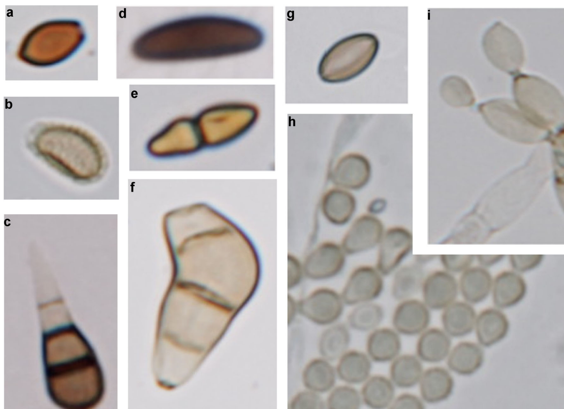
Fig. 2 Images of common fungal spores sampled at the different heights over the rainforest and identified up to family level. a Agaricaceae, b Polyporaceae, c Pleosporaceae, d Xylariaceae, e Venturiaceae, f Pleosporaceae, g Agaricaceae, h Trichocomaceae, i Cladosporiaceae. Scale bar: 10 \mu\text{m} .
