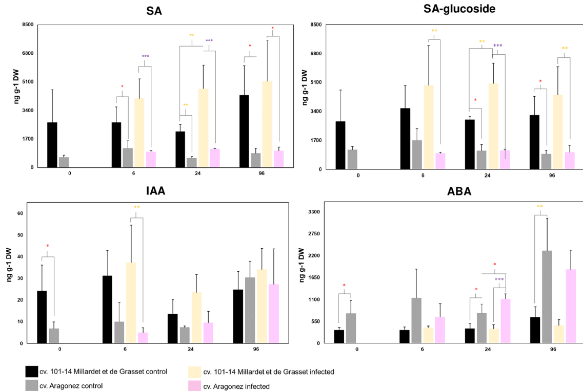
Fig. 2 Salicylic acid, IAA and Abscisic acid content in control and Powdery Mildew-infected grapevine leaves. Tolerant Vitis rupestris × riparia cv. 101-14 Millardet et de Grasset and susceptible Vitis vinifera cv. Aragonéz leaves were inoculated with Erysiphe necator and harvested at 0, 6, 24 and 96 h post-infection. Hormonal
