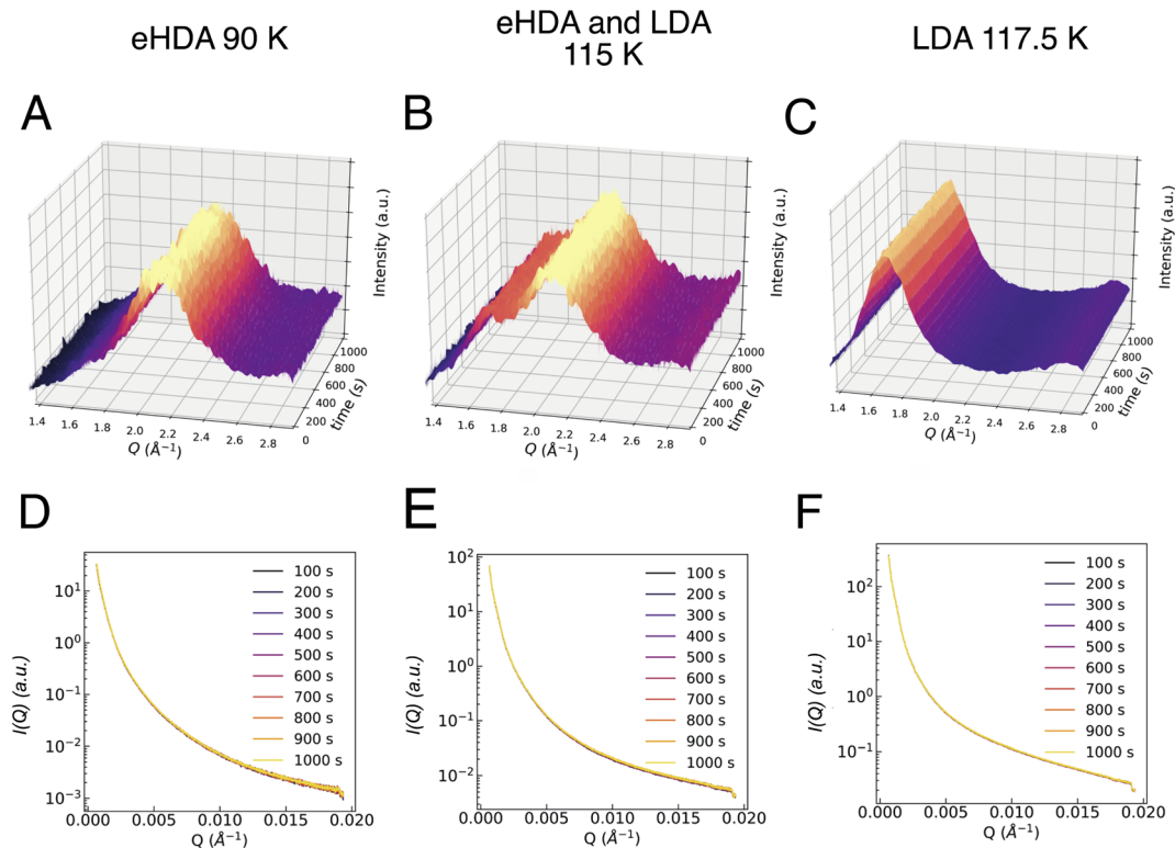
Fig. 2 Azimuthally integrated intensity in the WAXS geometry over 1000 s of (A) eHDA at 90 K, (B) eHDA transforming to LDA at 115 K, and (C) LDA at 117.5 K. The azimuthally integrated intensities in the USAXS geometry of the same samples are shown below (D, E and F, respectively). Each line corresponds to the average of 100 s. Therefore, the plot labelled as 100 s is the average for the first 100 s, the one labelled as 200 s is the average from 101 to 200 s, etc. Temperatures as measured at cold finger, T-sample might be slightly higher.
