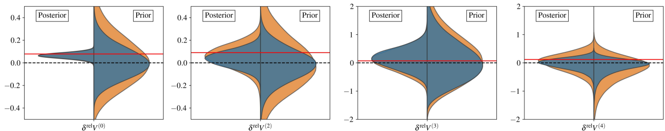
FIG. 5. Same MCMC results as in Fig. 4, but here we sample the relative errors of various derivatives of the effective potential \delta^{\text{rel}}V^{(n)} with respect to the tortoise coordinate evaluated at the maximum. The right side of each violin plot shows the sampling from the prior distribution of all \alpha^{(k)} simultaneously. The colors label the different \alpha^{(k)} prior ranges, \alpha_{P20}^{(k)} (blue) and \alpha_{P10}^{(k)} (orange). The left side of each violin plot shows the sampling from the posterior distributions, with colors labeling the prior assumptions. We mark the injections by horizontal red lines.
