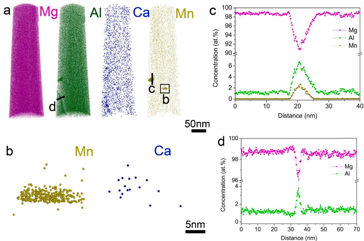
Fig. 8. 3D reconstruction of APT measurement for the rolled Mg-3Al-1Ca-Mn alloy within the material volume containing two nano-sized Al 8 Mn 5 particles. (a) distribution maps of Mg, Al, Ca, and Mn. (b) an enlarged Ca and Mn map from the marked area in (a) to show the Al 8 Mn 5 phase and a trace Ca segregation in the interface between Al 8 Mn 5 phase and Mg matrix. (c) 1D concentration profile measured by a cylinder of 2 nm in diameter (c) across the Al 8 Mn 5 phase (marked in Mn map in a) and (d) one grain boundary (marked in the Al distribution map in a).
