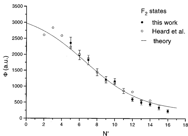
FIG. 7. A comparison of the present values for the relative quantum yield of OH ( A\ 2\Sigma^+ , v'=3 ) with the results of Heard et al. (Ref. 4) for F_1 states (a) and F_2 states (b). The smooth curves connect the calculated values by Yarkony (Ref. 5). The values are scaled to each other in F_2 , N'=11 .
