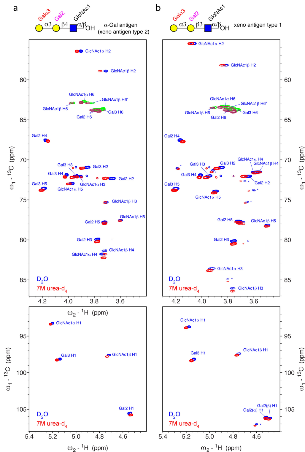
Figure 2. Chemical shift assignments of the \alpha -Gal antigen trisaccharide (Gal \alpha 1,3Gal \beta 1,4GlcNAc) and the xeno antigen type 1 trisaccharide (Gal \alpha 1,3Gal \beta 1,3GlcNAc) measured either in \text{D}_2\text{O} (blue) or in 7 M urea- \text{d}_4/\text{D}_2\text{O} at 298 K and pH* 7.4 (red). (a) Overlay of two ^1\text{H} - ^{13}\text{C} HSQC spectra of Gal \alpha 1,3Gal \beta 1,4GlcNAc measured either in \text{D}_2\text{O} (blue, with assignment) or in 7 M urea- \text{d}_4/\text{D}_2\text{O} pH* 7.4 (red). The spectra were recorded with multiplicity-editing leading to opposite sign for \text{CH}_2 groups (green and purple). The spectra were measured with 32 transients, a recycle delay of 1.5 sec and 2048 \times 512 points resulting in a total measurement time of 7.5 hours. A schematic presentation of the trisaccharide structure in its \alpha and \beta anomeric form is shown on the top. At the bottom the anomeric region of the ^1\text{H} - ^{13}\text{C} HSQC spectrum is shown. Few ^1\text{H} - ^{13}\text{C} three-bond correlations are visible as well (without label) in particular between H2-C3 and H3-C2 of Gal2 and Gal \alpha 3. (b) Overlay of two ^1\text{H} - ^{13}\text{C} HSQC spectra of related xeno antigen type 1 trisaccharide measured either in \text{D}_2\text{O} (blue, with assignment) or in 7 M urea- \text{d}_4/\text{D}_2\text{O} pH* 7.4 (red). The spectra were recorded with the same parameters as the \alpha -Gal antigen trisaccharide. Asterisks indicate signals of a minor impurity. Its identity and the chemical shift assignments are provided in the Supporting Information (Figure S2 and Table S2).
