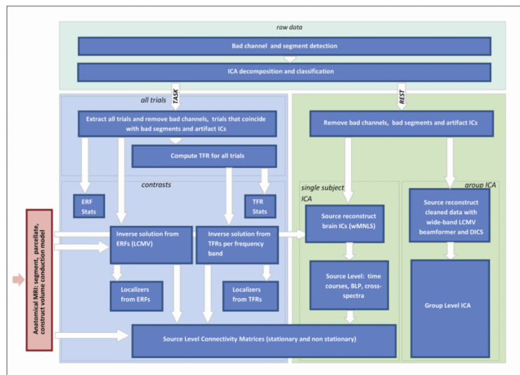
Figure 2. MEG Analysis Pipelines. The upper part of the pipeline labelled as “raw data” operates on the entire data set and is shared between the task and rest pipelines. For TASK (left panel), the box labelled as “all trials” operates on the concatenated epochs from all conditions; the box labelled “contrasts” operates on epochs of individual conditions and contrasts between conditions. For REST (right panel), the box labelled “single subject ICA” operates on temporal ICs at the individual level and the box labelled “group level ICA” operates on spatial ICA at the group level.
