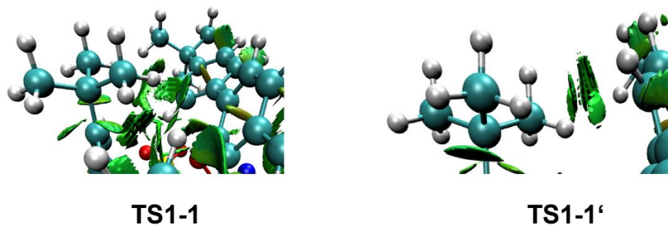
Figure S3. Noncovalent interactions of the t -Bu group of the BINOL aryl-substituent that does not form the catalyst pocket with the BINOL backbone ( 3b_1 , see Figure 5 ). It can be seen, that for TS1-1 additional dispersive interactions are present, which is why removal of this group leads do a relative stabilization of TS1-1' .
