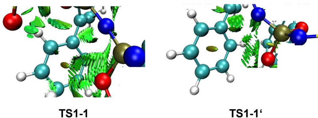
Figure S4. Noncovalent interactions of the Ph-ring bound to the BINOL substituent that is not forming the catalyst pocket ( 3b_2 , see Figure 5 ). Due to geometric distortion, TS1-1 is able to form stronger interactions with the catalyst's backbone, especially with the core catalyst's oxygen atom. Only for TS1-1 strong attractive interactions of this group are present. Its removal therefore energetically favors TS1-1' with respect to TS1-1 .
