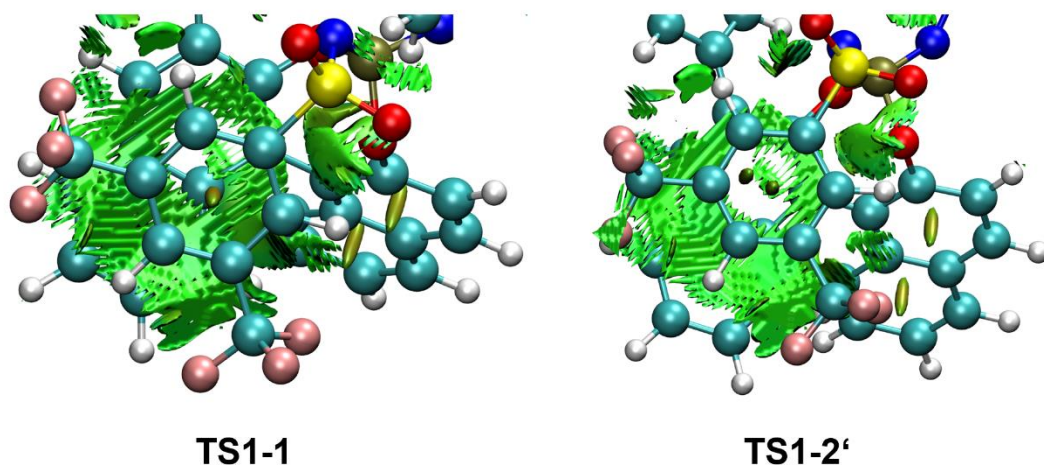
Figure S11. Noncovalent interactions between the iminyl-Ph-(CF 3 ) 2 -group with the residue ( 3b_4 , see Figure 5 ). For both TS conformers \pi - \pi interactions with the phenyl-rings of the residue are present, which is why the stereoselectivity is not affected by the removal of this group.
