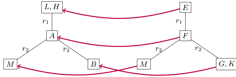
Fig. 3. Two description trees with a weak homomorphism between them.
