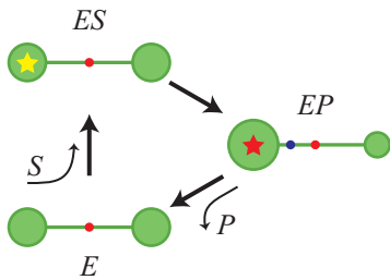
FIG. 1. Reaction cycle of the model dumbbell enzyme. The dumbbell consists of two beads connected by a link of a fixed length. Substrate S binds in the state E to domain 1 (left) and the substrate-enzyme complex ES is formed. In this state, rapid conversion of substrate into product P occurs, so that a transition to the product-enzyme complex EP takes place. After that, the product is released. The distance between the beads remains fixed, but the viscous friction coefficients of the beads are changed in the state EP . The RC and CM of the dumbbell are shown by red and blue dots, respectively. The two centers coincide in the states E and ES but they are shifted one from another in the state EP
