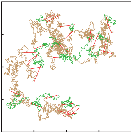
FIG. 3. The RC trajectory of the dumbbell over time t = 5 within the window of length \mathcal{L} = 4 (for \Delta\gamma = 0.8 , \kappa^{10} = 4 , \kappa^{01} = 10 , other parameters are given in the text). Fragments of the trajectory corresponding to the state s = 0 are shown as green, those corresponding to s = 1 are brown, and RC leaps in the transitions between the two states are displayed as red lines.
