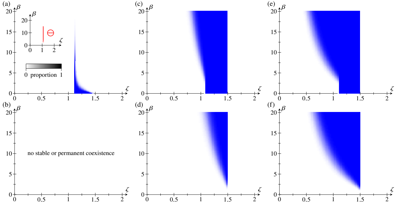
FIG. 7. Effect of the parameters \xi , \varpi , \varsigma on the stability and permanence of coexistence. Numerical stability and permanence results for Eqs. (4) if only one of the persister parameters \iota , \kappa , \mu , \xi , \varpi , \varsigma is nonzero: \xi > 0 [panels (a), (b)], \varpi > 0 [panels (c), (d)], \varsigma > 0 [panels (e), (f)]. Panels (a), (c), (e) have \eta/\alpha > \vartheta , while panels (b), (d), (f) have \eta/\alpha < \vartheta . Plots are analogous to and parameter values are equal to those in Fig. 6.
