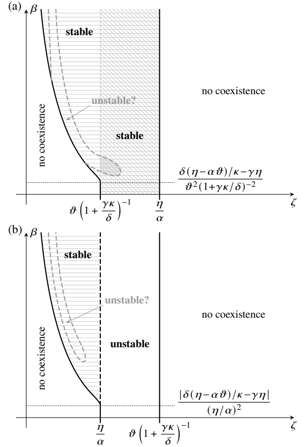
FIG. 13. Feasibility and stability of the coexistence states \mathcal{C}_{\pm} of the simplified model (B3) in the (\zeta, \beta) diagram for \kappa > 0 , in the cases (a) \eta/\alpha > \vartheta/(1 + \gamma\kappa/\delta) and (b) \eta/\alpha < \vartheta/(1 + \gamma\kappa/\delta) , assuming that the persister scalings (5) hold. Coexistence is feasible in the region bounded by the thick solid black lines. Both \mathcal{C}_+ and \mathcal{C}_- are unstable in the region marked “unstable”, but \mathcal{C}_- is stable (and \mathcal{C}_+ is unstable) in the region marked “stable”. Whether \mathcal{C}_- is unstable in a subregion of the “stable” region must be determined numerically. In the diagonally hatched region of parameter space in panel (a), the trivial steady states \mathcal{A} and \mathcal{B} are unstable, and the two species coexist permanently. If the “unstable” region intersects this region, all steady states of Eqs. (B3) are unstable within this intersection. The horizontally hatched region is the region of stable steady-state coexistence for averaged models of Eqs. (B3) without phenotypic variation and with stochastic switching only; coexistence may be stable in the average with respect to \mathcal{C}_- and in that with respect to \mathcal{C}_+ (Appendix C).
