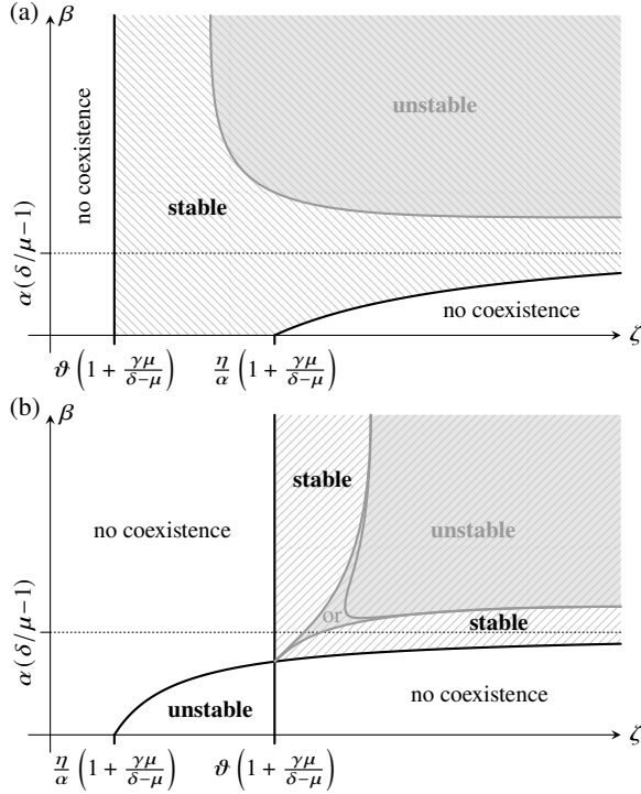
FIG. 12. Feasibility and stability of the coexistence state \mathcal{C} of the simplified model (B2) in the (\zeta, \beta) diagram for \mu > 0 , in the cases (a) \eta/\alpha > \vartheta and (b) \eta/\alpha < \vartheta . Coexistence is feasible in the region bounded by the thick solid black lines, and is stable or unstable in the regions marked “stable” or “unstable”, respectively. A region of instability (grey lines) arises at sufficiently large \beta, \zeta . The exact boundary of this region must be computed numerically. Equations (B37) and (B38c) express the necessary and sufficient conditions for the two different behaviors (“or”) that are possible in panel (b). In the hatched region of parameter space, the trivial steady states \mathcal{A} and \mathcal{B} are unstable, and the two species coexist permanently. The solidly hatched region in panel (a) is also the region of stable steady-state coexistence for an average of Eqs. (B2) without phenotypic variation and with stochastic switching only (Appendix C); the dashed hatching in panel (b) signifies that steady-state coexistence cannot be stable in the averaged model for \eta/\alpha < \vartheta (Appendix C). In the shaded regions of parameter space, all steady states of Eqs. (B2) are unstable.
