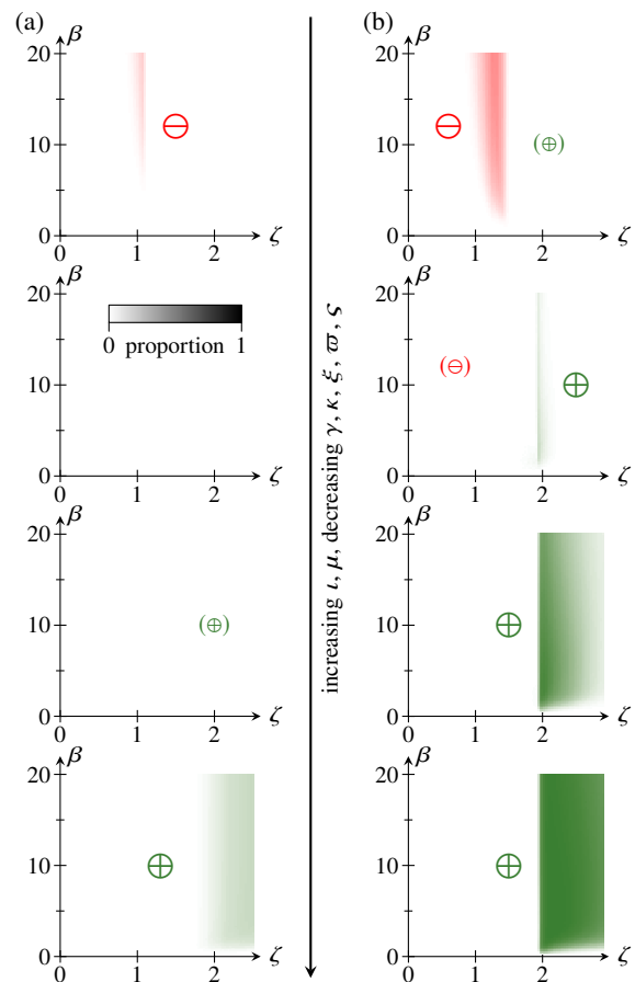
FIG. 8. Stabilization of coexistence by “elevated” persister growth \mu or persister-competitor interaction \iota . Plots, in (\zeta, \beta) space and for (a) \eta/\alpha > \vartheta and (b) \eta/\alpha < \vartheta , of the proportion of N = 1000 random instantiations of Eqs. (4) for which coexistence is stabilized (or becomes permanent), \oplus , or destabilized, \ominus , compared to the averaged model with stochastic switching only. Proportions are represented by the colors of the points in the diagrams, with symbols in parentheses indicating that the stability or permanence of a proportion of systems too small to be visualizable by the color scheme changes compared to the averaged model. The “elevation” of \iota, \mu increases from top to bottom. Parameter values: \alpha = 0.8, \eta = 1.2 , (a) \vartheta = 1.1 or (b) \vartheta = 1.9 , and \delta \sim \mathcal{U}[0.8, 1.6] , as in Figs. 5–7; also, \gamma, \mu, \xi, \varpi, \varsigma \sim \mathcal{U}[\varepsilon/f, 2\varepsilon/f] , \mu, \iota \sim \mathcal{U}[\varepsilon f, 2\varepsilon f] , with \varepsilon = 0.1 and where f \in \{1 \text{ (top)}, 1.5, 2, 2.5 \text{ (bottom)}\} “elevates” the values of \iota, \mu .
