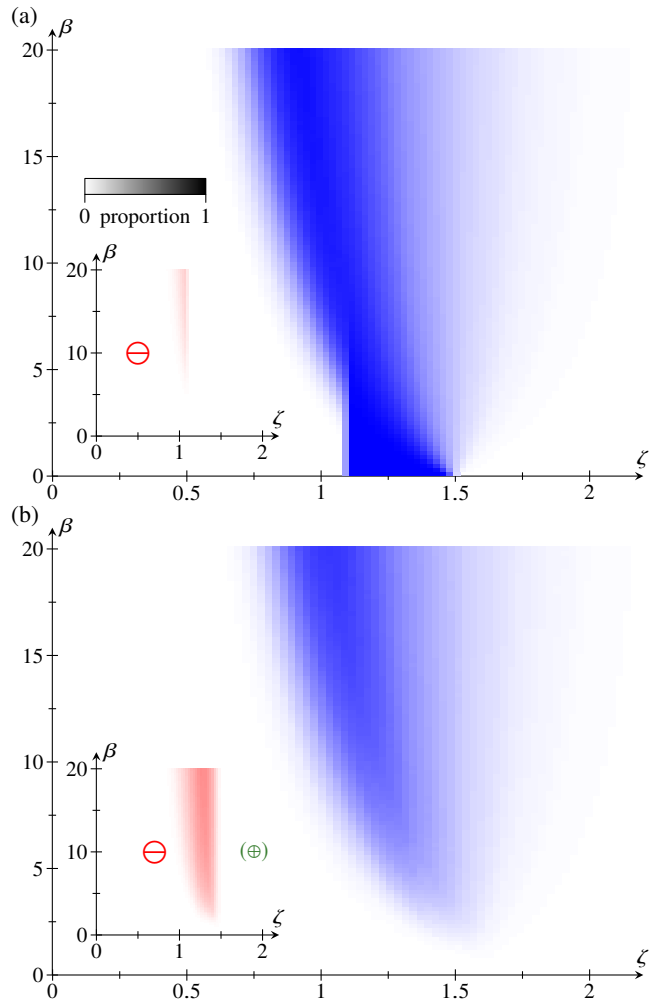
FIG. 5. Numerical stability diagrams of Eqs. (4) in the (\zeta, \beta) diagram in the cases (a) \eta/\alpha > \vartheta and (b) \eta/\alpha < \vartheta . The color of each point in the stability diagrams represents the proportion of N = 1000 random systems for which coexistence is stable or permanent at that point. The insets plot the proportion of systems for which coexistence is destabilized, \ominus , compared to the averaged model with stochastic switching only. The symbol \oplus in parentheses [panel (b), inset] indicates that a nonzero proportion of systems (too small to be visualizable by the color scheme) is stabilized (or becomes permanent) compared to the averaged model. Parameter values: \alpha = 0.8 , \eta = 1.2 , \vartheta = 1.1 [panel (a)] or \vartheta = 1.9 [panel (b)], \gamma, \iota, \kappa, \mu, \xi, \varpi, \varsigma \sim \mathcal{U}[\varepsilon, 2\varepsilon] , with \varepsilon = 0.1 , and \delta \sim \mathcal{U}[0.8, 1.6] .
