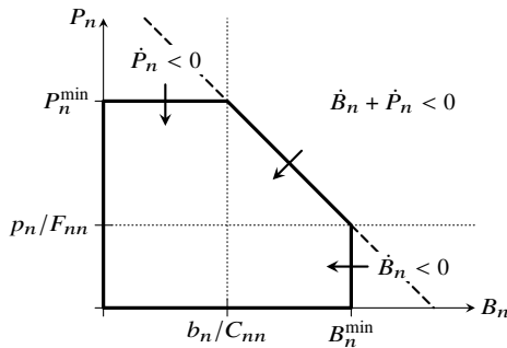
FIG. 9. Bounded dynamics of Eqs. (1). For any nonnegative initial conditions, (B_n, P_n) will eventually enter the pentagonal bounding region (thick lines), and remain in that region for all times. If C_{nn} = 0 and b_n < \varepsilon k_n or F_{nn} = 0 and p_n < \ell_n , the sides of the bounding region are modified (dashed lines).
