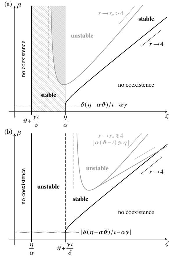
FIG. 11. Feasibility and stability of the coexistence states \mathcal{C}_{\pm} of the simplified model (B1) in the (\zeta, \beta) diagram for \iota > 0 , in the cases (a) \eta/\alpha > \vartheta + \gamma\iota/\delta and (b) \eta/\alpha < \vartheta + \gamma\iota/\delta , assuming scalings (5). Coexistence is feasible in the region bounded by the thick solid black lines. Both \mathcal{C}_+ and \mathcal{C}_- are unstable in the region marked “unstable”, but \mathcal{C}_- is stable (and \mathcal{C}_+ is unstable) in the region marked “stable”. The exact boundary of the region of instability that arises at sufficiently large \beta (grey lines) must be computed numerically; a region of stability at large \zeta, \beta must exist in case (a), but only exists in case (b) if \alpha(\vartheta - \iota) < \eta . The boundary of this region asymptotes to the straight line \beta\iota/\alpha\delta\zeta \equiv r = r_* , where r_* is defined in Eq. (B21b) and depends only on \alpha(\vartheta - \iota)/\eta . In the hatched region of parameter space, the trivial steady states \mathcal{A} and \mathcal{B} are unstable, and the two species coexist permanently. This is also the region of stable steady-state coexistence for an average of Eqs. (B1) with respect to \mathcal{C}_- without phenotypic variation and with stochastic switching only (Appendix C). In the shaded region of parameter space (which need not exist), all steady states of Eqs. (B1) are unstable.
