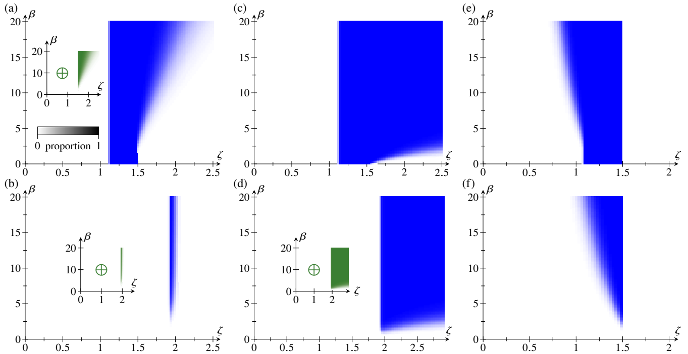
FIG. 6. Effect of the parameters \iota , \mu , \kappa on the stability and permanence of coexistence. Numerical stability and permanence results for Eqs. (4) if only one of the persister parameters \iota , \kappa , \mu , \xi , \varpi , \varsigma is nonzero: \iota > 0 [panels (a), (b)], \mu > 0 [panels (c), (d)], \kappa > 0 [panels (e), (f)]. The analytical results in Appendix B confirm some of these results. The cases \eta/\alpha > \vartheta [panels (a), (c), (e)] and \eta/\alpha < \vartheta [panels (b), (d), (f)] lead to qualitatively different diagrams. The color of each point in the stability diagrams represents the proportion of N = 1000 random systems for which coexistence is stable or permanent at that point. The insets similarly plot the proportion of systems for which coexistence is stabilized (or becomes permanent), \oplus , or destabilized, \ominus , compared to the averaged model with stochastic switching only; there is no (de)stabilization where there is no inset. Parameter values: \alpha = 0.8 , \eta = 1.2 , and \vartheta = 1.1 [panels (a), (c), (e)] or \vartheta = 1.9 [panels (b), (d), (f)]. The remaining parameters (if not set to zero) were sampled uniformly and independently, constrained by the persister scalings (5): \gamma, \iota, \kappa, \mu, \xi, \varpi, \varsigma \sim \mathcal{U}[\varepsilon, 2\varepsilon] , with \varepsilon = 0.1 , and \delta \sim \mathcal{U}[0.8, 1.6] .
