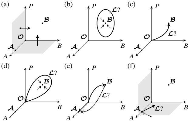
FIG. 10. Permanent coexistence of the two species described by Eqs. (B1) if \mathcal{A}, \mathcal{B} are unstable. (a) Orbits of Eqs. (B1) are expelled from B = 0 and P = 0 . (b) Non-existence of a (stable) limit cycle \mathcal{L} in \Pi = \{A = 0; B, P > 0\} . (c) Non-existence of a connection \mathcal{L} containing \mathcal{B} in \Pi . (d) Non-existence of a homoclinic connection of \mathcal{O} in \Pi . (e) Non-existence of a connection containing \mathcal{O} \rightarrow \mathcal{B} . (f) Non-existence of a connection containing \mathcal{A} , because one of the connections of \mathcal{A} is not feasible.
