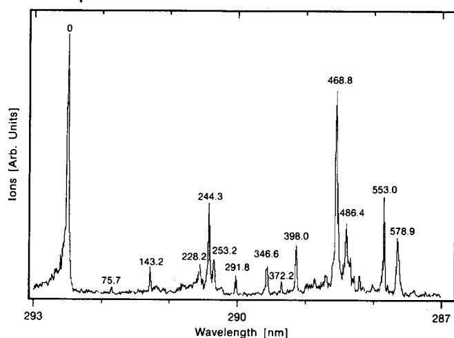
FIG. 13. (1 + 1)-REMPI spectrum of the PABA-CH 3 OH hydrogen bonded complex, recorded at mass 169. Frequency distances of the various vibrations from the origin are indicated with a \pm 1 \text{ cm}^{-1} accuracy. The origin of this complex is 16.3 \pm 0.7 \text{ cm}^{-1} blueshifted from the PABA origin.
