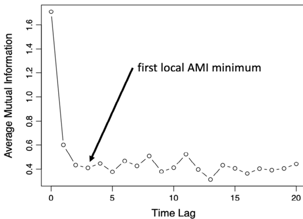
Fig. 5 Average mutual information (AMI) values for the first 20 time lags of the synthetic IKI data. A first local minimum is visible at lag 3
