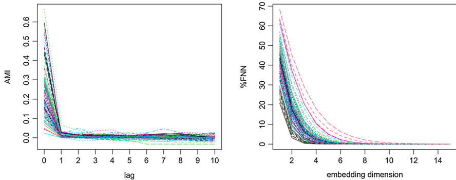
Fig. 9 The average mutual information (AMI) function (left) and false nearest neighbors (FNN) function (right) for each time series revealed a delay parameter t = 1 and an embedding parameter m = 7
