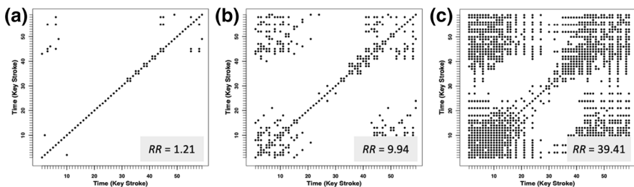
Fig. 7 Effects of the threshold parameter r on recurrence plots for the putative inter-key interval data and the resulting recurrence rate (RR). RQA was computed with a delay parameter t=3 , an embedding dimension parameter m=5 , and the threshold parameters a r=0.01 , b r=1.5 , and c r=2.5
