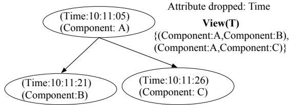
Fig. 6: Simple trace and an example of a view
