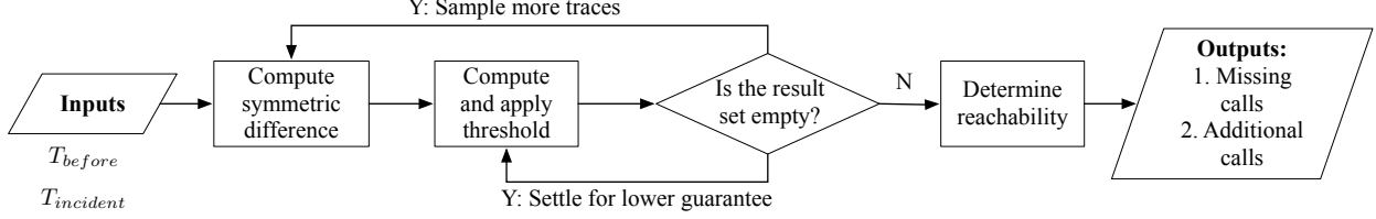
Fig. 7: ACT consists of applying three techniques: Symmetric difference, thresholding and reachability - in that order.
