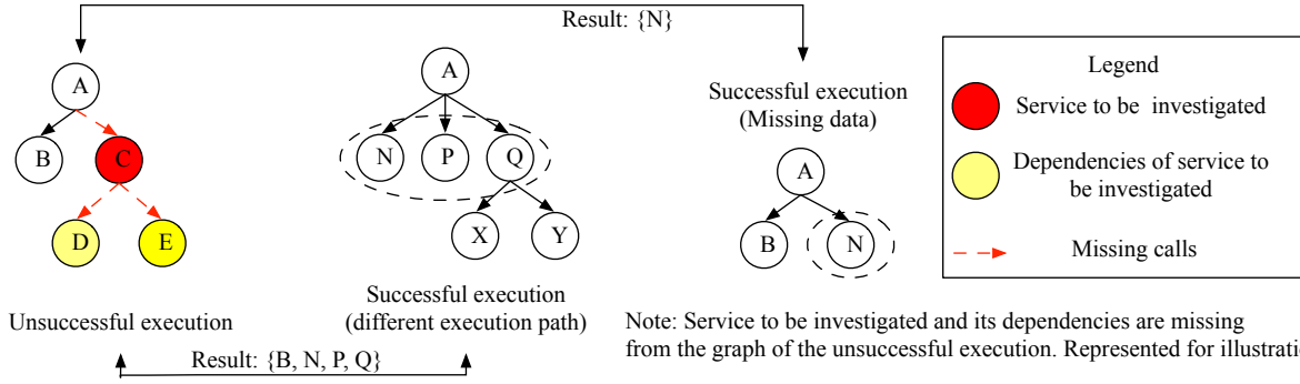
Fig. 5: Limitations of pairwise comparison - the two examples demonstrate the circumstances when pairwise comparison produces false alarms and can occur either separately or in combination.
