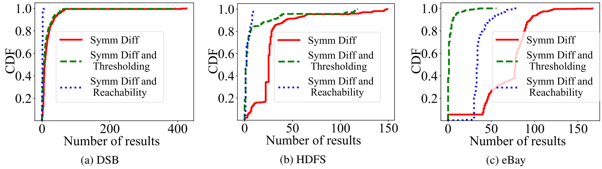
Fig. 10: CDFs of the number of results returned when we apply one or two techniques. Since the eBay dataset is noisy, symmetric difference and thresholding performs best, while symmetric difference and reachability generate the best results for DSB and HDFS. When all three techniques of ACT are applied, the result is obtained is exactly the mitigation site.
