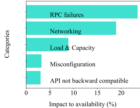
Fig. 1: Percentage of impact by category - we have represented the top five of over a dozen different categories that emerged based on available data. Incidents arising due to breakdown in communication between components at the application level have the highest impact.
