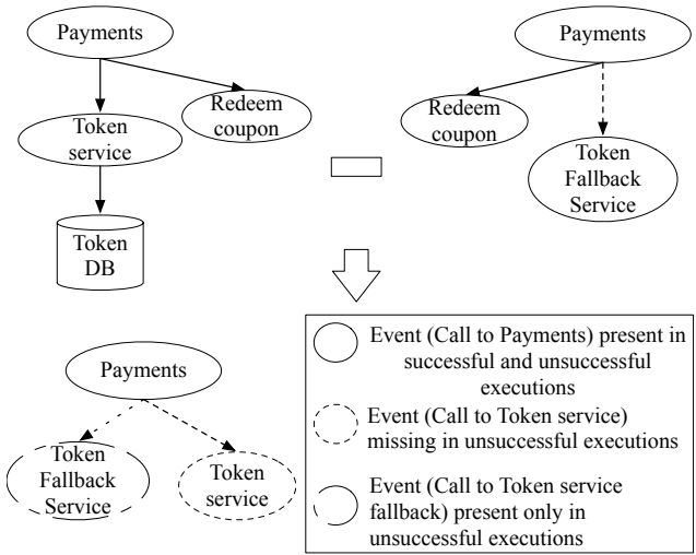
Fig. 4: This figure represents an idealized picture of graph differencing and contains only the relevant services. On the left is a partial view of a successful request where the token service was working as expected. On the right, we have the trace, after the restart of the payments service which continued to see errors due to incorrect firewall rules.
