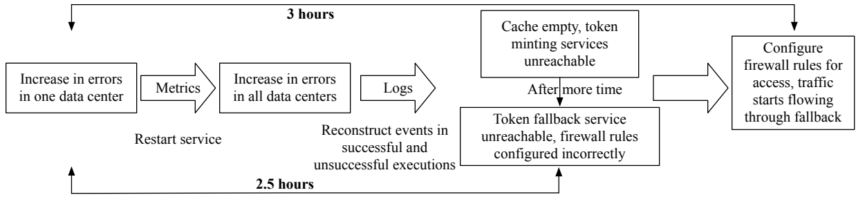
Fig. 3: This figure represents how SREs responded to an incident and the data sources they used (logs and metrics). The mitigation steps took SREs close to three hours, two and half of which was arriving at the correct mitigating action.
