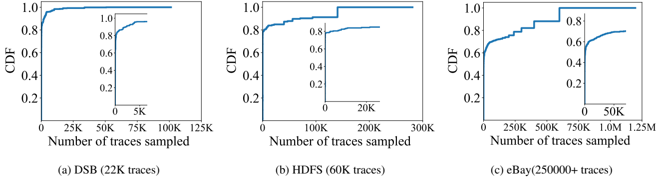
Fig. 8: CDF of the number of traces to be sampled to identify any possible missing edge. The inlaid snippet of the CDF shows that a majority of calls can be identified with a sample that is orders of magnitude smaller.
