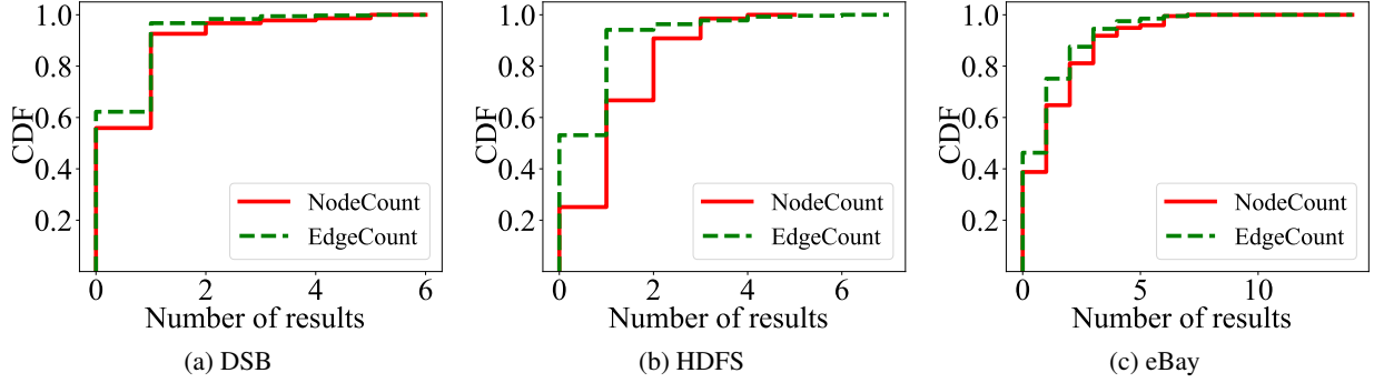
Fig. 9: For the cases when NodeCount and EdgeCount produce results, we plotted a CDF of number of results. ACT, meanwhile, produces exactly the expected answer for all of these cases.
