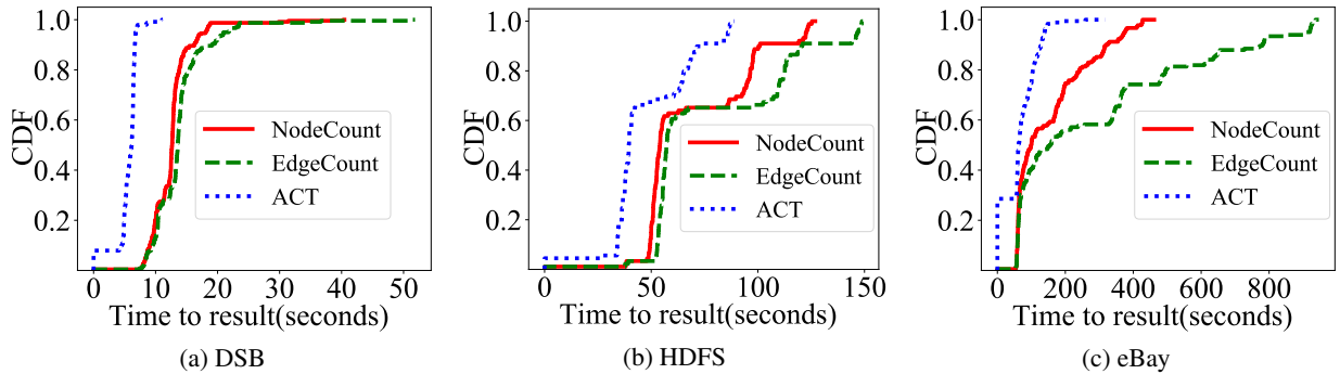
Fig. 11: CDFs of time taken to obtain a result. Reachability accounts for most of the time taken by ACT . Nodecount and Edgecount have highly variable time to result since trace of every unsuccessful execution needs to be compared with that of every successful execution and the number of unsuccessful executions can vary widely.
