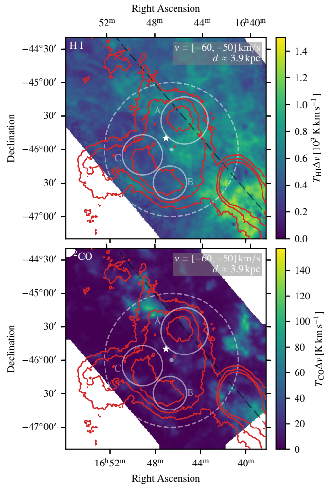
Fig. 8. Maps showing H I emission (McClure-Griffiths et al. 2005) (top panel) and ^{12}\text{CO} emission (Braiding et al. 2018) (bottom panel) in the Westerlund 1 region. Both maps display the emission for an interval in velocity with respect to the local standard of rest of v = [-60, -50] \text{ km s}^{-1} , which approximately corresponds to a distance of 3.9 kpc. The position of Westerlund 1 is marked by the white star symbol and the grey, dashed line shows the Galactic plane. The transparent, white circle marker denotes the centre point with respect to which the radial CR density profiles in Fig. 9a have been computed; the dashed white line displays a circle with radius 1^\circ – up to which the profiles have been computed – around this point. The red lines are contour lines of the flux map shown in Fig. 3a. Regions A, B, and C are the same as in Fig. 3.
