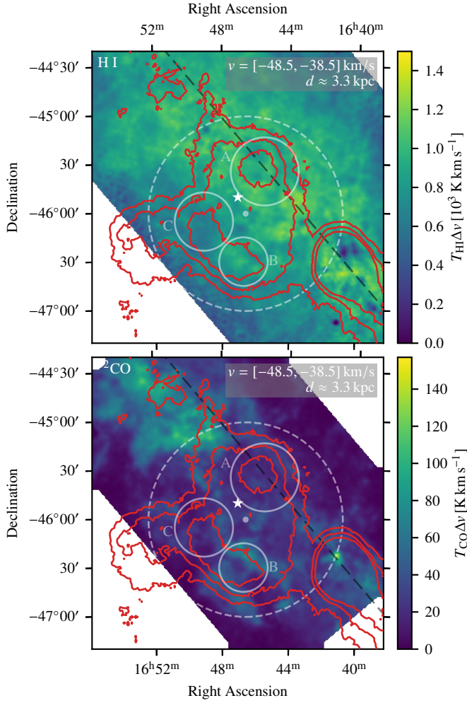
Fig. B.1. Same as Fig. 8, but adopting an interval in velocity with respect to the local standard of rest of v = [-48.5, -38.5] \text{ km s}^{-1} .
