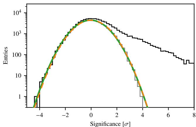
Fig. 2. Significance entry distribution. The black histogram corresponds to all pixels of the map shown in Fig. 1a with non-zero entries, the grey histogram to all pixels outside of the final exclusion map. The green line represents the fit of a Gaussian distribution to the grey histogram, the best-fit mean and width are \mu = -0.043 \pm 0.005 and \sigma = 1.008 \pm 0.005 , respectively. A Gaussian distribution with mean \mu = 0 and width \sigma = 1 is shown by the orange, dashed line for comparison.
