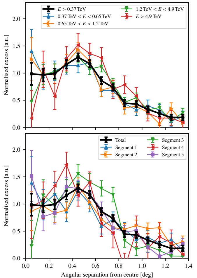
Fig. 4. Radial excess profiles. The upper panel shows exposure-corrected excess counts per unit sky area for different energy bands, the lower panel for different segments as defined in Fig. 1b – the black curve, showing the total excess above threshold in all segments, is the same in both panels. All profiles are normalised to equal area, to allow an easy comparison. The profiles have been computed with respect to a centre point at R.A. 16^{\text{h}}46^{\text{m}}36^{\text{s}} , Dec. -46^\circ01'12'' , slightly shifted from the Westerlund 1 position. In the calculation of the profiles, we discarded pixels within 0.6^\circ of the position of HESS J1640–465.
