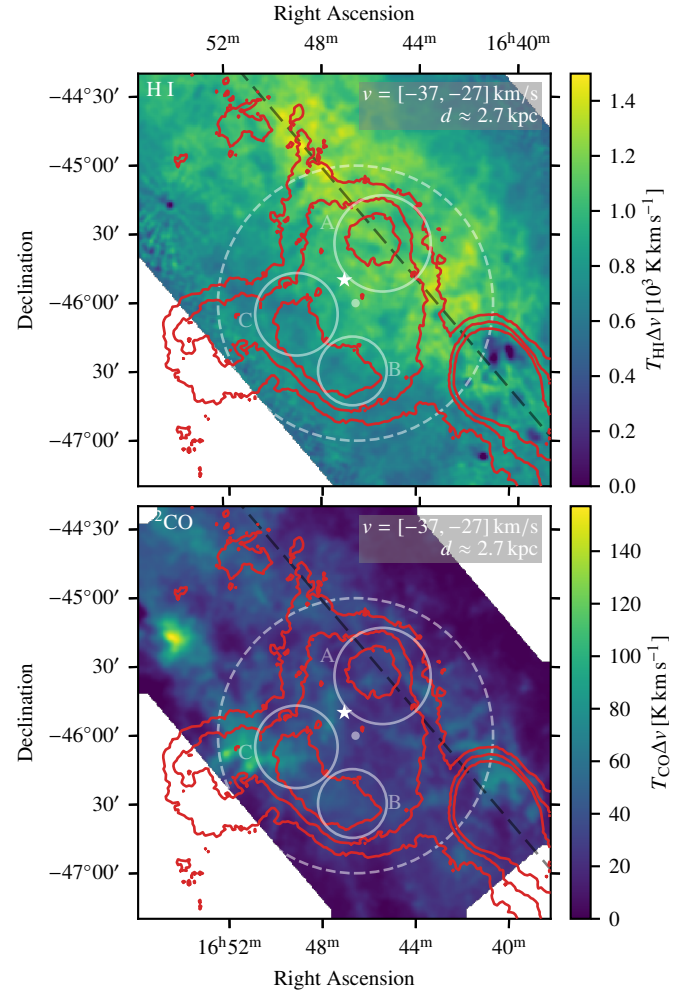
Fig. B.2. Same as Fig. 8, but adopting an interval in velocity with respect to the local standard of rest of v = [-37, -27] \text{ km s}^{-1} .
