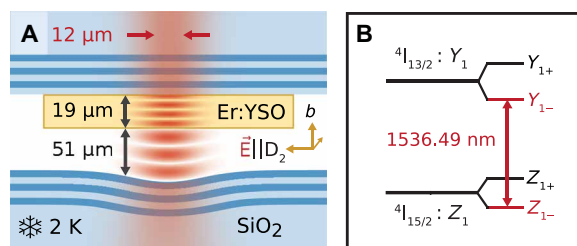
Fig. 1. Setup and level scheme. (A) Fabry-Pérot cavity (not to scale). A resonator with small mode volume is formed by a flat and a concave glass mirror (blue; bottom and top) with deposited Bragg reflectors (dark blue), confining a stable optical mode (red). Erbium dopants are integrated in a thin, atomically flat crystalline membrane (yellow rectangle). (B) Energy level scheme. The studied transition (red) is between the lowest spin and crystal-field levels of the 15/2 and 13/2 manifolds of erbium in YSO.
