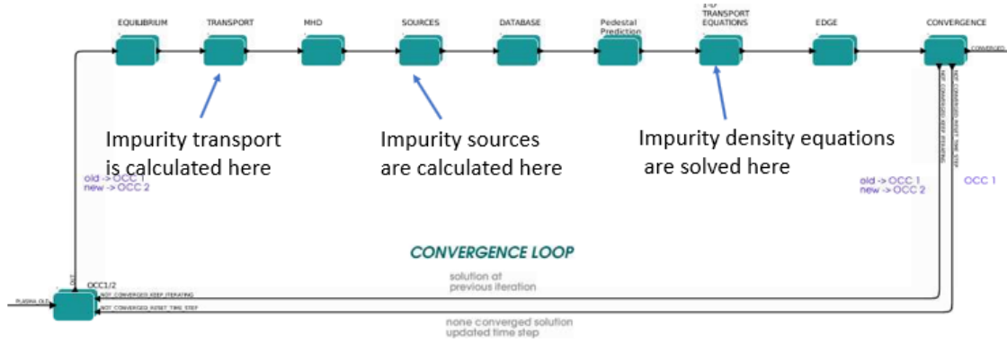
Figure 1: Kepler layout of the ETS Convergence Loop with indication of the modules relevant to the impurity density equations
