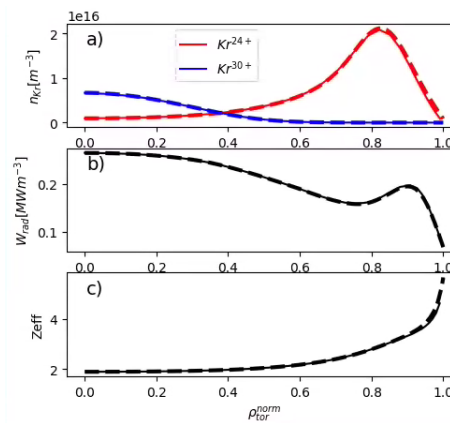
Figure 5: Results ETS/SANCO for Kr after 2 sec of simulation time. a) state densities; b) radiation power density; c) Z_{eff} . Solid - SANCO, dashed - ETS
