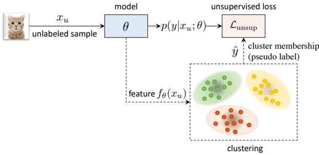
Fig. 11: In unsupervised discriminative models using deep clustering (§3.2.2), unlabeled samples are assigned to a set of clusters by online or offline clustering, while the cluster memberships are utilized as pseudo labels for training.
