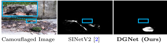
Fig. 9 Hard sample with small camouflaged object.
