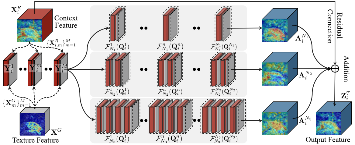
Fig. 4 Illustration of the proposed gradient-induced transition (GIT).
