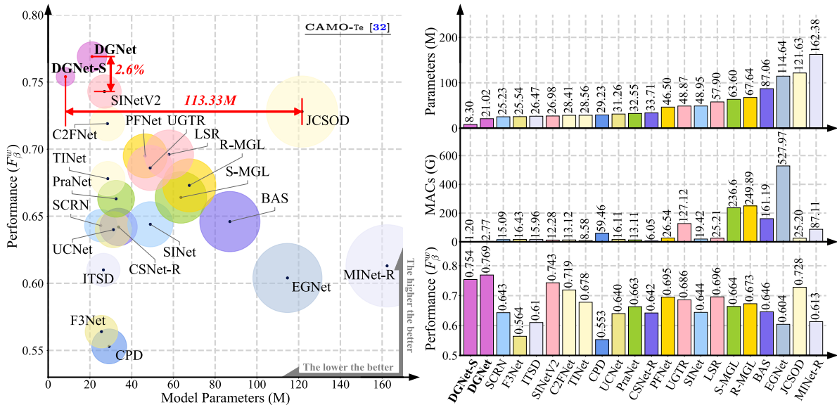
Fig. 7 (Left) We present the scatter relationship between the performance ( F_{\beta}^w ) and parameters of all competitors on CAMO-Te [32]. The larger the colored scatter point size, the heavier the model parameters. (Right) We also report the parallel histogram comparison of model’s parameters, MACs, and performance ( F_{\beta}^w ). Best viewed in color.
