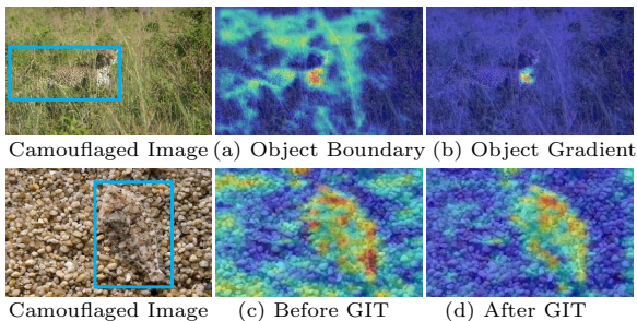
Fig. 8 Feature visualizations of two core designs, including the supervision of object gradient (1 st row) and the GIT (2 nd row).
