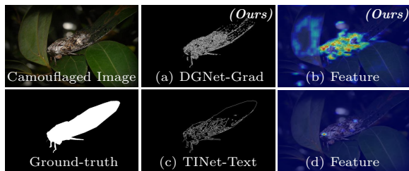
Fig. 2 Compared to the texture label proposed in TINet [36], our object gradient label (a) keeps more geometric cues inside the camouflaged object. DGNet under the supervision of texture label (c) fails to infer attentive regions (d) since the imbalanced distribution of sparse pixels ( e.g. , thin object boundaries). Notably, such improvement exerts our DGNet more robust with the reliable auxiliaries, e.g. , feature in (b).
