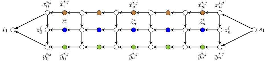
Figure 5: The paths X^{i,j} , Z_i and Y^{i,j} are shown. If the index of a vertex is a , then its weight is M if the vertex is blue, Ma if the vertex is brown, M(n+1-a) if the vertex is green and W+1 otherwise. This gadget together with the definition of the target weight W of the solution, ensures that a solution picks exactly one vertex from each of the three paths. Moreover, the three vertices chosen from these three paths have the same index.
