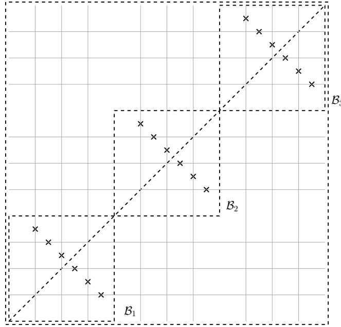
Figure 3: The set \mathcal{M}_3 . The meeting points are represented by crosses. The dashed lines indicate the sides of the large square and of the k -boxes.
