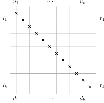
Figure 2: A 6-box. The meeting points are represented with crosses. Thus, every line contains two segments of the box, whose only intersection is the meeting point on this line.
