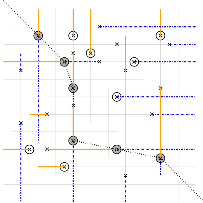
Figure 1: Selection of the two independent sets in the proof of Lemma 3. Crosses are the meeting points, disks are the candidate points, and gray disks are the cut points. The black dotted line is the cut. Dashed blue and solid orange segments are those chosen to the sets S_{\text{blue}} and S_{\text{orange}} , respectively.
