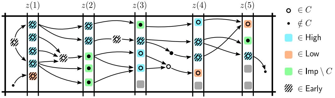
■ Figure 4 Figure presents a schedule with five sink moments z(1), \dots, z(5) . Jobs from Vertex Cover are marked with a black ring (the remaining jobs are depicted with a black-filled circle). Set \text{Imp} contains every job in the sink-moment (highlighted either blue, green or red). Jobs from \text{High} are highlighted in blue. Jobs from \text{Low} are highlighted red. Jobs from \text{Imp} \setminus C are highlighted green. Early jobs are wrapped with a solid black border. Gray rectangles are empty slots in the schedule. Observe that for a fixed chain there exists a single moment after which every job in it is late. This moment corresponds to the job from \text{Imp} \setminus C on this chain.
