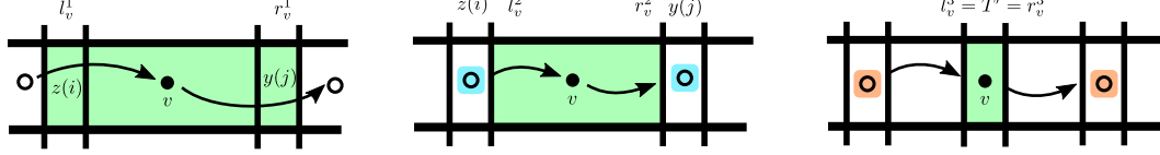
■ Figure 7 Schematic picture of determining lower bounds l_v^1, l_v^2, l_v^3 and r_v^1, r_v^2, r_v^3 . We highlighted green the available intervals (e.g., [l_v^1, r_v^1] ) of job v . The first schema determines l_v^1 and r_v^1 . For example, if vertex u is in block B_i then l_v^1 \geq z(i) . Middle schema says that if v has predecessor from High in sink-moment z(i) then l_v^2 > z(i) . Last condition simply says that if a sink in V(\sigma_L) is predecessor of v then it needs to be processed at T' or later. Inequalities for l_v^4 and r_v^4 are similar to the last figure.
