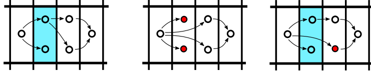
■ Figure 3 Examples of three schedules with makespan 4 and m = 2 . The sink-moments are highlighted in blue. Only the left schedule is sink-adjusted. The middle schedule is not sink-adjusted because the red jobs are sinks and are scheduled before a non-sink. The right schedule is not sink-adjusted because the red job is not a predecessor of any job in a trailing sink-moment.
