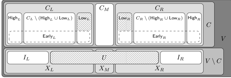
■ Figure 5 Venn diagram of the sets often used in Section 4. Recall that by definition I_L = \text{pred}(C_L) \setminus C_L and I_R = \text{succ}(C_R) \setminus C_R . The dashed area is equal to U' , defined in Subsection 4.3.
