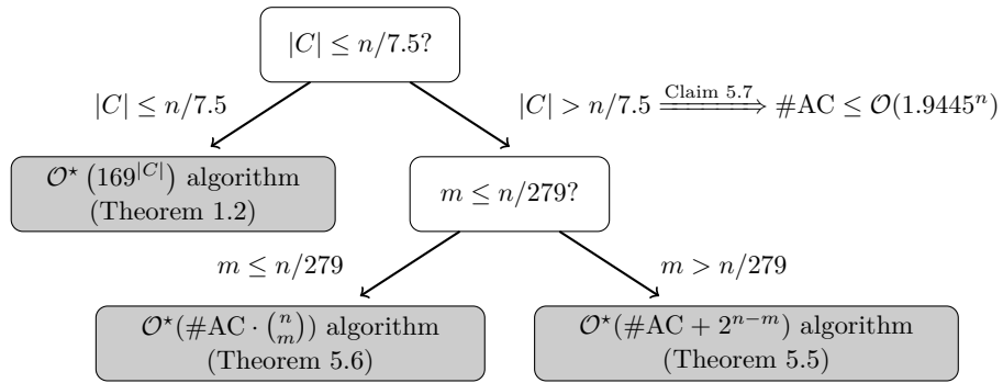
■ Figure 1 Overview of use of algorithms for proving Theorem 1.1.
