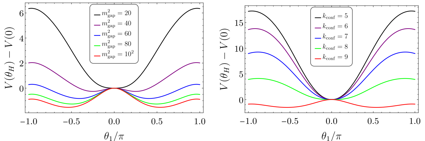
FIG. 10. The IR potential at the \theta_2 = 0 plane in a confinement-emulated scenario. Left: Various values of m_{\text{gap}}^2 with k_{\text{conf}} = 9 fixed. Right: Various values of k_{\text{conf}} with m_{\text{gap}}^2 = 10^2 fixed.
