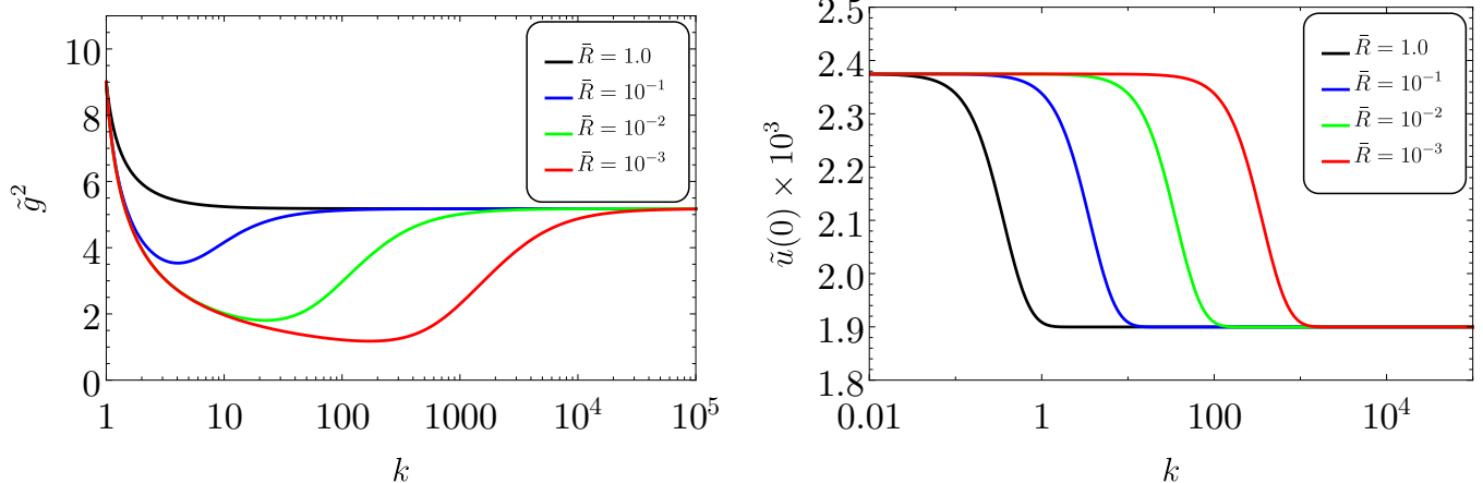
FIG. 8. Flow of the gauge coupling \tilde{g}^2 (left) and the vacuum energy (right) for several fixed values of the dimensionless compactification radius \bar{R} . The energy unit of k is arbitrary.
