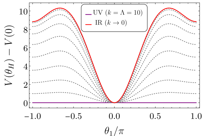
FIG. 2. The renormalization group evolution of the potential V(\theta_H) - V(0) at the \theta_2 = 0 plane (with \theta_3 = -\theta_1 - \theta_2 ) from the UV to IR scales. The energy units of k are arbitrary. Each dotted line corresponds to the potential at a lowered scale by \Delta k = 1 .
