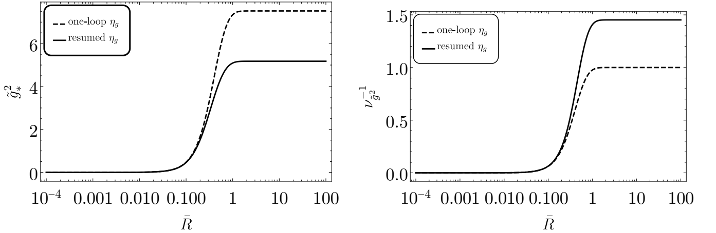
FIG. 5. The nontrivial fixed point value \tilde{g}_*^2 (left) and the critical exponent \nu_{\tilde{g}_*}^{-1} (right) of the gauge coupling as a function of the dimensionless compactification radius \bar{R} .
