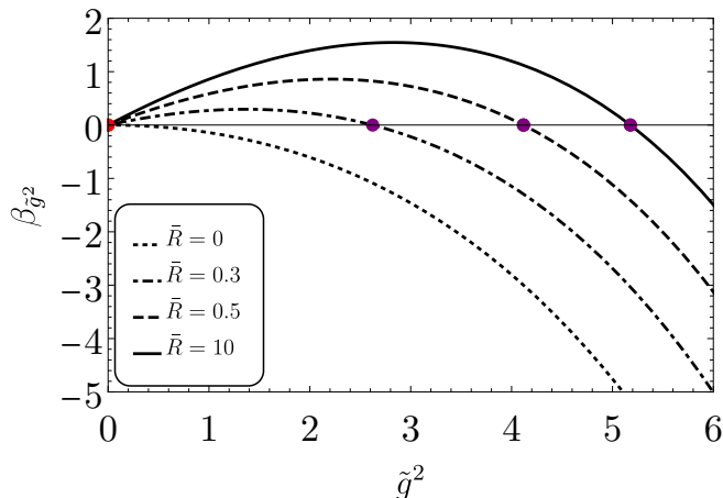
FIG. 6. The one-loop beta function of \tilde{g}^2 as a function of \tilde{g}^2 . The purple points stand for the nontrivial fixed point, while the red point indicates the Gaussian fixed point.
