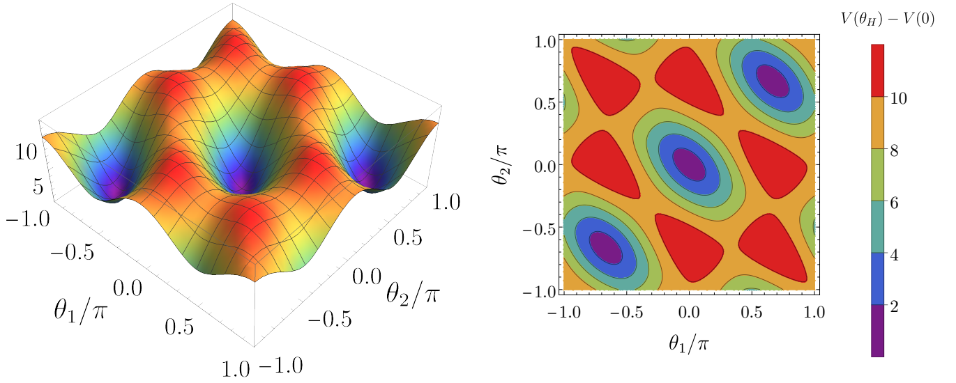
FIG. 3. 3 dimensional plot (left) and contour plot (right) of the potential V(\theta_H) - V(0) at the IR scale ( k \rightarrow 0 ). Note \theta_3 = -\theta_1 - \theta_2 .
