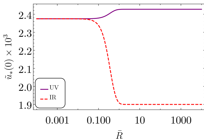
FIG. 7. The nontrivial UV (solid purple line) and IR (dashed red line) fixed point values as a function of the dimensionless compactification radius \bar{R} .
