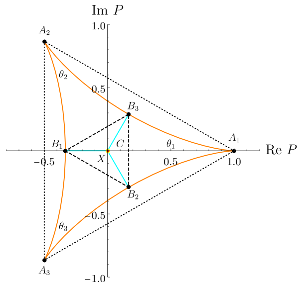
FIG. 1. Configurations of the Polyakov loop. We set \alpha = \pi/3 , \beta_1 = 0 and \beta_2 = 2\pi/3 . The horizontal and vertical axes correspond respectively to the real and imaginary parts of the Polyakov loop. The configurations names are listed in Table I.
