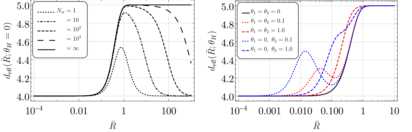
FIG. 4. The effective dimension d_{\text{eff}} as a function of the dimensionless compactification radius. Left: Dependence of d_{\text{eff}} on truncation limits on the KK mode summations as |n| = N_{\text{tr}} in the symmetric phase ( \theta_1 = \theta_2 = \theta_3 = 0 ). Right: The effective dimension with the full resummation of KK modes for the different AB phases shown in Table I. Note \theta_3 = -\theta_1 - \theta_2 .
