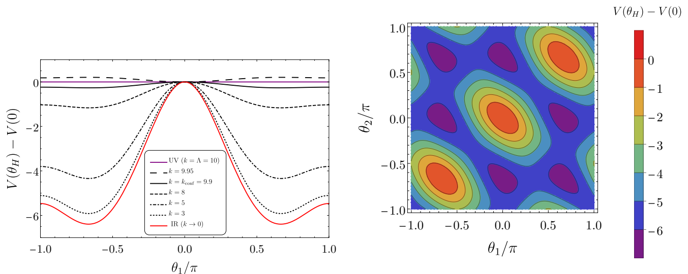
FIG. 9. The potential with m_{\text{gap}}^2 = 10^2 and k_{\text{conf}} = 9.9 in a confinement-emulated scenario. Left: The renormalization evolution of the potential at the \theta_2 = 0 plane from \Lambda = 10 to k = 0 . Right: Contour plot of the potential at the IR scale k \rightarrow 0 in \theta_1 - \theta_2 plane.
