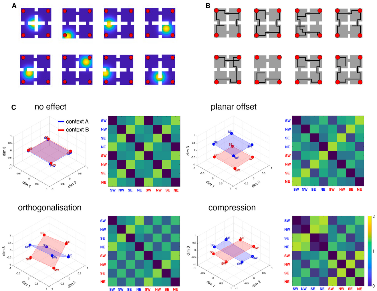
Figure 2. Computational modeling
