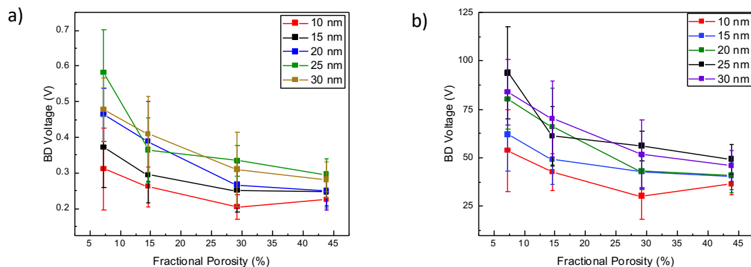
Figure 6.9. Evaluation of breakdown voltage of the device under poling condition in a) air, and b) vacuum.
