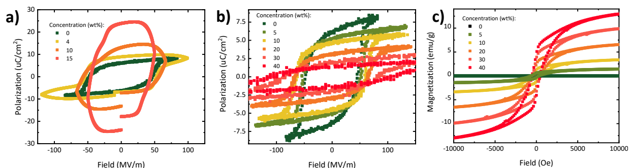
Figure 8.9. Polarization and magnetization characterization of the nanocomposite thin films. Polarization, P - E , response of the nanocomposite thin films of P(VDF-TrFE) with a) as-synthesized nanoparticles and b) PMMA-grafted nanoparticles with various loadings. c) Magnetization, M - H , response of the nanocomposite thin films using PMMA-coated nanoparticles at different loadings.
