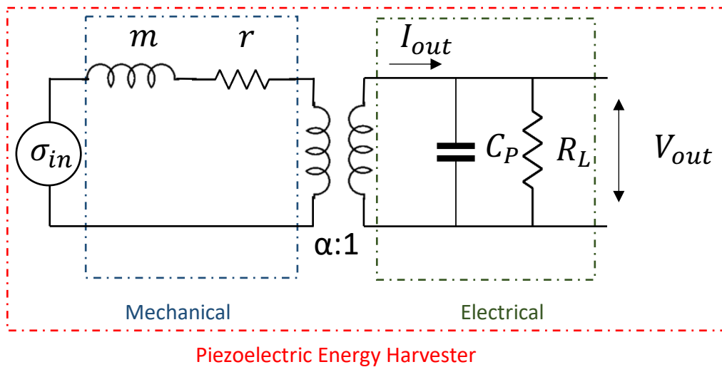
Figure 5.1. systemic electric model of a piezoelectric energy harvester, two mutually coupled inductors represent the coupled nature of mechanical and electrical properties of piezoelectric materials.
