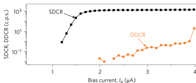
Fig. 9 Plot of the system dark count rate due to background photons (SDCR, black) and the device dark count rate (DDCR, orange) of a typical fiber-coupled SNSPD. Note that near 4 μA the switching current is reached. Adapted with permission from ref. 46. Copyright 2013 Nature Publishing Group.
