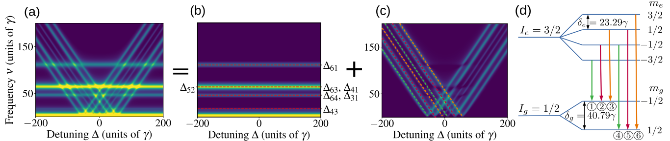
FIG. 2. Decomposition of FFC spectra into single-target and two-target contributions. (a) shows the real part of the FFC spectrum \mathcal{I}(\nu, \Delta) after removal of the off-resonant background. It can be separated into two parts shown in (b) and (c). The first part in (b) is the sum of the individual responses of target and analyzer, corrected for the non-resonant absorption. The horizontal structures are due to quantum beats in the target. As guide to the eye, the relevant mutual detunings between the target transitions are indicated by dashed red lines. (c) is the difference between the spectra in (a) and (b). This spectrum is dominated by diagonal structures, which originate from the interference of the resonant scattering off of the different target resonances with the resonant analyzer response. These results are obtained for a 2\mu\text{m} thick enriched \alpha - {}^{57}\text{Fe} target with hyperfine field B = 33.3 T and a stainless-steel single-line analyzer as described in the main text. The level structure and the relevant transitions in the target are shown in (d). The orange, red and green transitions describe the scattering of left-circularly, linearly and right-circularly polarized light, respectively.
