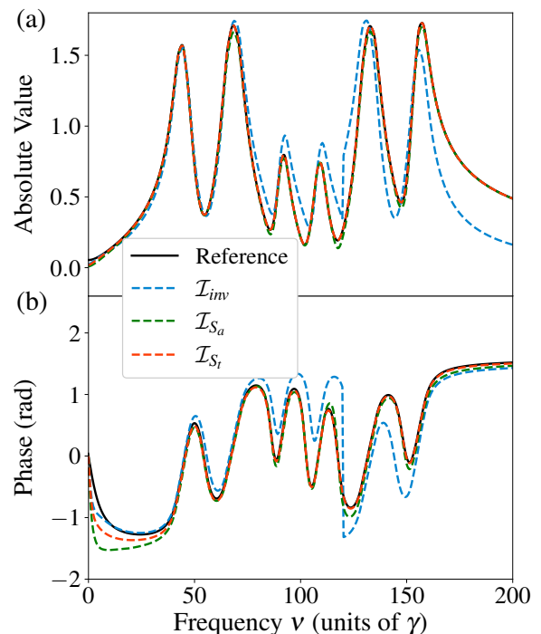
FIG. 12. Reconstruction of the nuclear resonant target response from phase-combined FFC spectra: (a) depicts the absolute value of a vertical cut through the FFC spectra at \Delta = 100\gamma (dashed lines). For comparison, the absolute value of the reference nuclear resonant response correlated with the analyzer response according to eq.(16) is shown as solid black line. (b) shows the corresponding phase of the quantities shown in (a). The blue line corresponds to the background-corrected sum spectrum \mathcal{I}_{inv} while the green and orange line correspond to the cases with the analyzer ( \mathcal{I}_{S_a} ) and the target ( \mathcal{I}_{S_t} ) placed first in the beam path, respectively.
