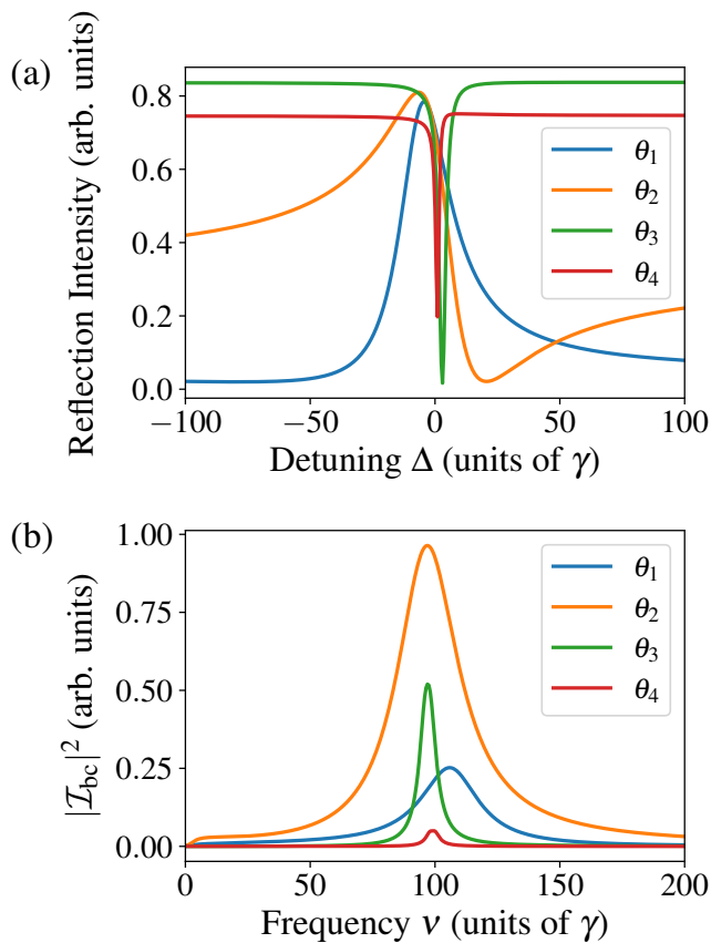
FIG. 6. Cavity spectra for different x-ray incidence angles \theta_1 = 2.75\text{mrad} , \theta_2 = 2.8\text{mrad} , \theta_3 = 3.0\text{mrad} and \theta_4 = 3.3\text{mrad} . (a) shows full reference cavity reflection spectra calculated using the software package PYNUSS. The effect of the electronic scattering on the cavity structure is clearly visible in the off-resonant background varying with the incidence angle, and in the modification of the Lorentzian nuclear response into a Fano line profile. (b) shows the nuclear target response recovered from the FFC spectrum by vertical sections at \Delta = 100\gamma (cf. yellow line in Fig. 5). These spectra are not affected by the electronic scattering on the cavity, and therefore remain of Lorentzian shape for all incidence angles. Therefore, the dependence of the superradiant line broadening and the resonance energy shift on the incidence angle become clearly visible.
