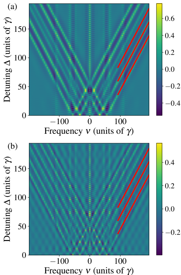
FIG. 9. Effect of time gating on the extraction of target parameters from the diagonals in the FFC spectra. The two panels show FFC spectra as in Fig. 3, but with initial time vetos of (a) 20 ns and (b) 40 ns. In both cases, only times up to an upper limit of 192 ns are considered. Although the Fourier effects due to the time windows are clearly visible, the data can still be reliably fitted with lines of slope one, as indicated by the red lines.
