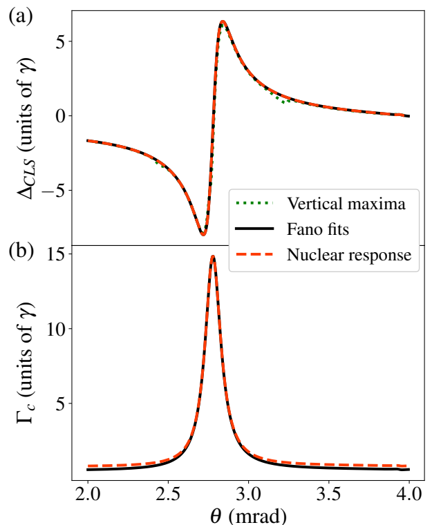
FIG. 7. Collective nuclear parameters of the two-level system realized by the cavity structure in Fig. 5. (a) shows the energy shift of the nuclear resonance related to the collective Lamb shift as function of the x-ray incidence angle, and (b) the corresponding superradiantly enhanced decay rate. The red dashed lines are the recovery results obtained from fitting a model to the FFC spectrum (see main text for details). The green dashed line in (a) is obtained using a simple maximum determination. As a reference, the solid black line shows the parameters obtained via a Fano line fit to the reference cavity spectrum calculated using PYNUSS.
