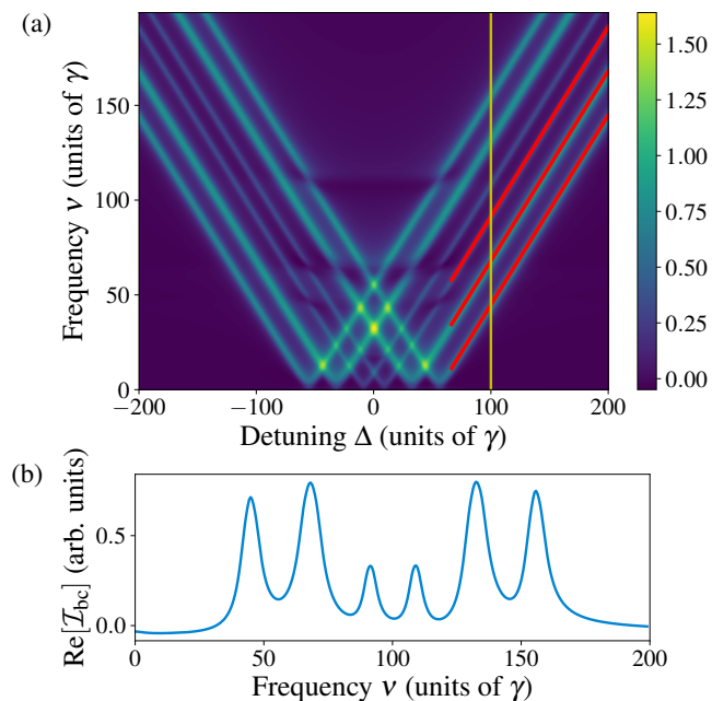
FIG. 3. Extraction of spectral parameters via linear fits to the diagonal structure. (a) shows the real part of the FFC spectrum for a 2\mu\text{m} thick \alpha -iron enriched in ^{57}\text{Fe} probed in Nuclear Forward Scattering (see main text for details). The analyzer is a stainless steel foil as described in the main text. The diagonal structure is clearly visible. The line fits used to extract the resonance positions are marked in red. (b) shows a vertical cut through (a) at a detuning \Delta = 100\gamma . This detuning is indicated by the yellow vertical line in (a). The six resonances of the magnetically split \alpha -Fe spectrum can clearly be distinguished.
