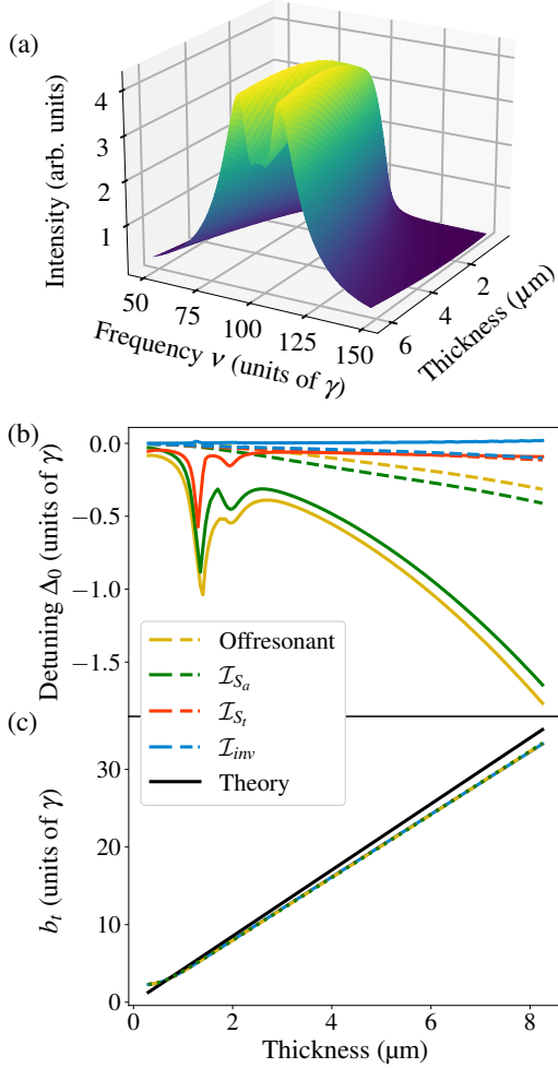
FIG. 11. Extraction of target parameters as function of target thickness. Panel (a) illustrates how the diagonal structure along the \nu -axis at \Delta = 100\gamma varies with target thickness. For thicker targets, a characteristic “double-hump” profile appears. (b) compares the deviations between the reference transition frequency and the corresponding transition frequencies obtained by linear fits to the diagonals using different methods: The off-resonant method (yellow line), and the phase-difference methods based on \mathcal{I}_{S_a} (green), \mathcal{I}_{S_t} (red) and \mathcal{I}_{inv} (blue). In all cases, the solid lines correspond to results obtained by simple maxima determination while the dashed lines are based on model fits to vertical sections through the diagonal structure, as explained in the main text. (c) compares the thickness parameters extracted from the different methods with the theoretical reference value (black).
