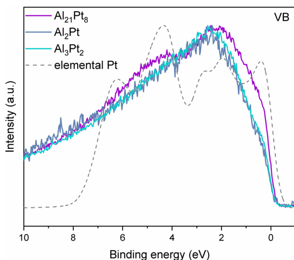
Fig. 6 Normalized XPS spectra of the valence bands for \text{Al}_{21}\text{Pt}_8 , \text{Al}_2\text{Pt} and \text{Al}_3\text{Pt}_2 after 2 h of CP. The grey dashed line represents the calculated sum of the partial DOS for Pt, weighted by photoionization cross-section and broadened by a Gaussian of a full width at half maximum equal to 0.4 eV.
