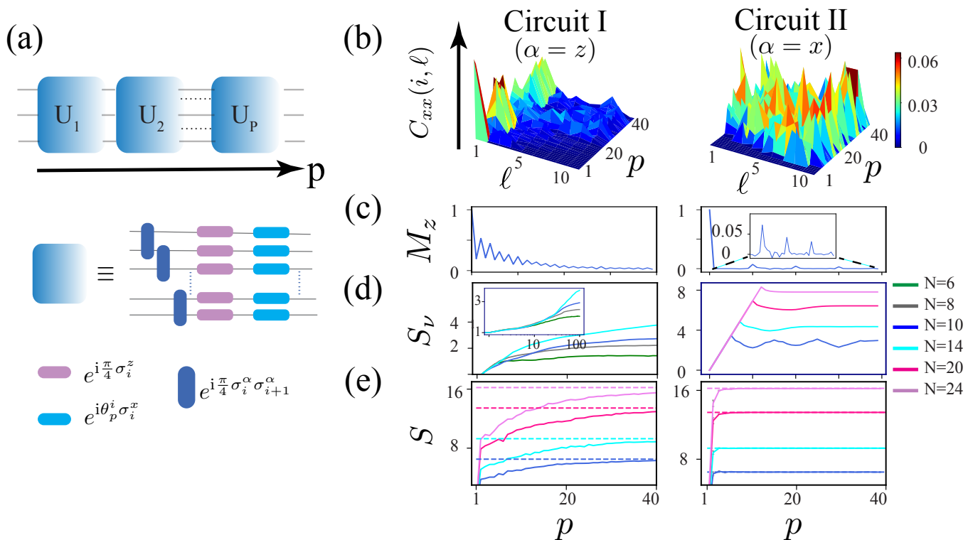
FIG. 1. Physical model: (a) Schematic representation of the random circuit. The circuit is made of modules shown as blue cells. Each module is made of three layers shown at the bottom. (b) Two-point correlators C_{xx}(i, \ell) = |\langle \sigma_{i+\ell}^x \sigma_i^x \rangle - \langle \sigma_{i+\ell}^x \rangle \langle \sigma_i^x \rangle|^2 versus circuit depth and distance \ell for the two different choices of two-body gates, circuit I (left) and circuit II (right), for N = 10 . (c)-(e) Magnetization, von-Neumann entropy, and entropy versus circuit depth for different system sizes for both, circuit I (left column) and circuit II (right column). Each curve represents an average over 20 circuit realizations. Dashed lines in panel (e) present the entropy of the ideal Porter-Thomas distribution. All shown results are for realizations of the circuits that are homogeneous in space, where C_{xx}(i, \ell) is the same for all qubits i .
