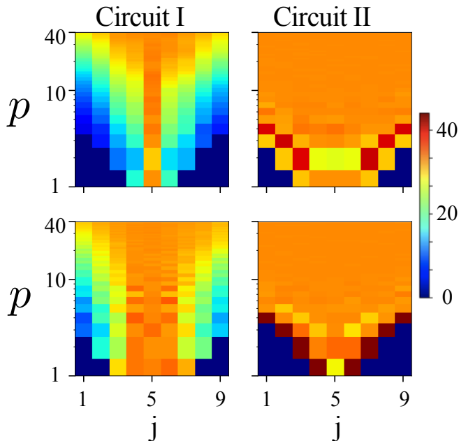
FIG. 6. Light-cone spreading of quantum information. The top panels show \|[\sigma_5^z, \sigma_j^z(p)]\|_F and the lower panels show \|[\sigma_5^x, \sigma_j^x(p)]\|_F for N = 9 averaged over 40 realizations for each panel. Both circuits are inhomogeneous in time and space ( \theta_p^i \neq \theta_p^j ).
