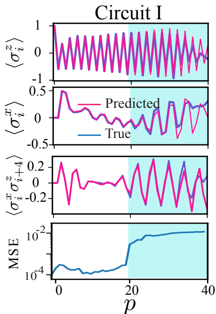
FIG. 4. Extrapolation power of the LSTM neural network in circuit depth for circuit I. The LSTM neural network is trained on the physical observables for random realizations of the circuit I on system size N = 8 with p \in [1, 20] . It is then evaluated on unseen realizations of the circuit with N = 8 and p \in [1, 40] . The performance of the network in generalization ( p \in [1, 20] ), as well as extrapolation in circuit depth (highlighted with blue, p \in [20, 40] ) for a typical realization of the circuit, is shown. The lower right panel shows the MSE averaged over 1000 realizations of the circuit. For each realization of the circuit, the neural network is trained on 40 observables simultaneously. The circuit is chosen to be homogeneous in space ( \theta_p^i = \theta_p^j ), hence \langle \sigma_i^z \rangle , \langle \sigma_i^x \rangle and \langle \sigma_i^x \sigma_{i+4}^z \rangle are equal for all qubits i .
