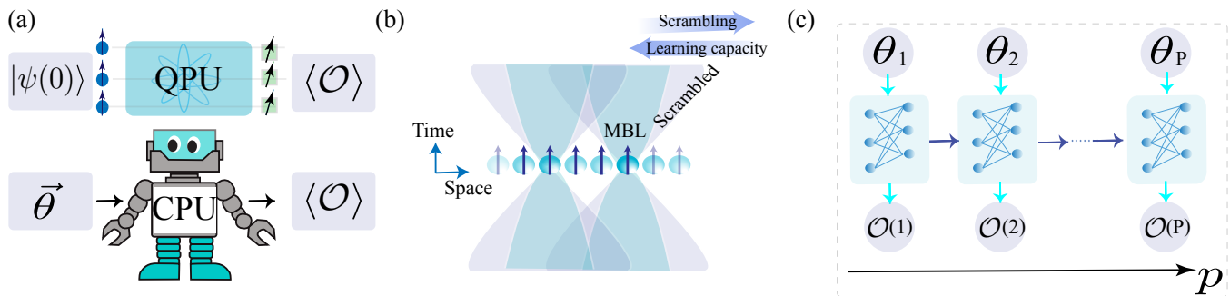
FIG. 2. Schematic representation of the applied learning strategy. (a) The neural network learns a simple and efficient representation for the equations of motion when provided with the parameters of the model (shown with \vec{\theta} ) just by observing a subset of physical observables, but without knowing the unitary operator that describes the model. (b) The propagation of information in a many-body system forms a light cone. For MBL models the radius of the light cone grows logarithmically while it propagates polynomially for scrambled models. Two qubits do not affect each other if one lies outside of the light cone of the other. The representation learned by the neural network is reliable beyond the system size and time window that it has been trained on where information scrambles slowly (logarithmically) and the dynamics is localized. (c) Schematic representation of the LSTM neural network. The input of the network at each circuit depth p is a set of random parameters \theta_p . At each circuit depth p the network provides as output the dynamics of desired observables \langle \mathcal{O}(p) \rangle . The horizontal blue arrows indicate the content of the internal neural memory being passed to the next time step.
