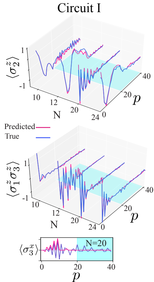
FIG. 5. Extrapolation power of CONVLSTM in system size and circuit depth for circuit I. The network is trained on system size N = 8 and p \in [1, 20] on the dynamics of desired observables and evaluated on unseen samples N = 10, 12, 20, 24 with p \in [1, 40] . The performance of the network in predicting a few observables is shown. The neural network is trained on inhomogeneous (both in time and space) realizations of circuit I ( \theta_p^i \neq \theta_p^j ).
