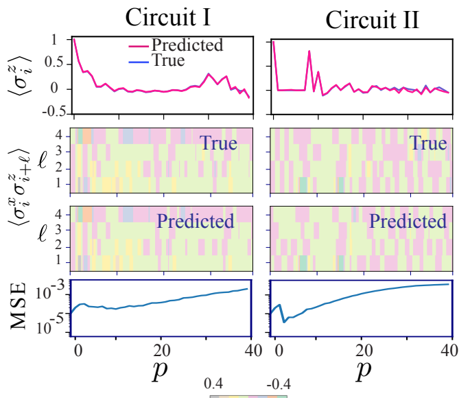
FIG. 3. Generalization power of the LSTM network: The neural network is trained separately on random realizations of both circuits with N = 8 and p \in [1, 40] . It is then evaluated in predicting the dynamics of observables on unseen realizations of the network in predicting \langle \sigma_i^z \rangle and \langle \sigma_i^x \sigma_{i+\ell}^z \rangle for a typical realization of both circuits is shown. The lower panels show the MSE, c.f. Eq. (2) as an over 1000 realizations of the circuit. For each realization of the circuit, the neural network is trained on 40 observables simultaneously. Both circuits are chosen to be homogeneous in space ( \theta_p^i = \theta_p^j ).
