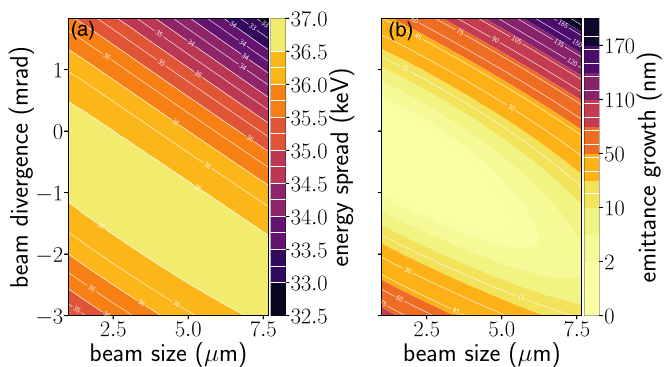
FIG. 5. Electron beam matching into a low-power [ E_z(r = 0) \sim 12 MV/m] laser-driven fiber with an excited TM_{01} mode in a 6 mm long ARF. The 2D parameter scan of the initial beam size at the structure entrance [ \sigma_r(z = 0) ] and the correlated beam divergence ( \sigma_r' ) is shown. The resulting energy spread and normalized emittance growth are displayed in (a) and (b), respectively.
