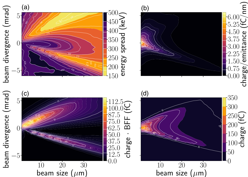
FIG. 6. Electron beam matching into a laser-driven fiber with an excited TM_{01} mode in a 6-mm-long ARF; the maximum on-axis accelerating field is E_z = 180 MV/m. The 2D parameter scan of the initial beam size at the structure entrance [ \sigma_r(z = 0) ] and the correlated beam divergence ( \sigma_r' ) is shown. The final beam properties after the collimator (placed 1 m downstream) are illustrated in the scans: energy spread (a), charge over normalized emittance (b), charge times the bunch form factor (c), and charge (d). Good matching regions are observed with large energy spreads, little emittance growth, and large charge transmission.
