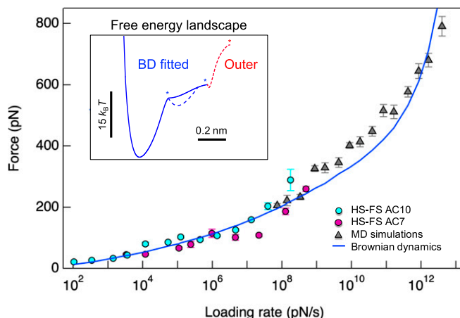
Fig. 2. Dynamic force spectrum of SA/b unbinding. Most probable rupture forces (± SEM) from HS-FS experiments (circles, using regular AC10 and fast AC7 cantilevers, cyan and magenta, respectively) and MD simulations (triangles). The blue line represents a Brownian dynamics fit to the whole force spectrum. (Inset) The resulting equilibrium free-energy landscape is shown as a blue line, which revealed two transition barriers (with parameters D = 4 \times 10^7 \text{ nm}^2/\text{s} , \Delta G_1 = 17 \text{ k}_B T , \Delta G_2 = 21 \text{ k}_B T , x_{\beta 1} = 0.19 \text{ nm} , and x_{\beta 2} = 0.44 \text{ nm} ) and a possible intermediate state between the two (blue dashed line). The red dashed line sketches a third, outer barrier (Fig. 3 and text), which cannot be extracted from the dynamic force spectrum.
