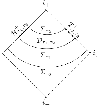
FIGURE 1. Hyperboloidal foliation and related definitions.
