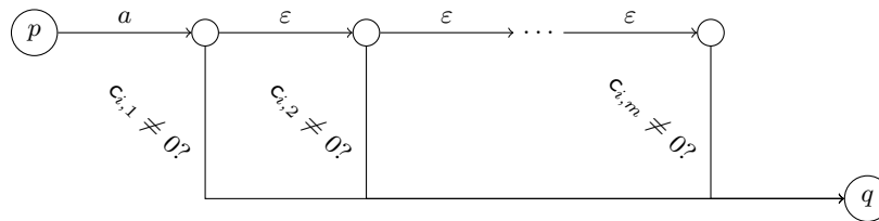
Fig. 4. Transition structure to replace a non-zero-test (p, a, \text{nz}_i, q) .
