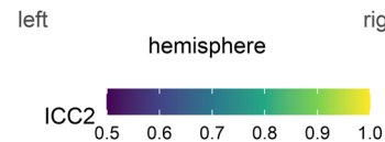
Fig. 3. ICC2 estimates across structural measures and brain regions. Lighter colours indicate higher stability.
