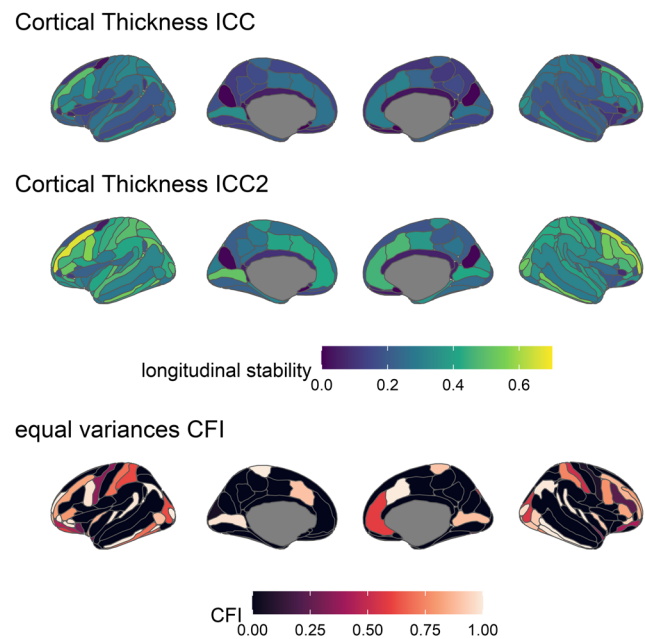
Fig. 10. ICC (top), ICC2 (middle), and CFI estimates for the constrained (error variances equal between timepoints) ICED model (bottom) for cortical thickness across brain regions (Destrieux parcellation). For ICC estimates (top and middle), lighter colours indicate higher stability. Note that for clarity we shifted the scale compared earlier in ICC (Figs. 2, 3, and 9). For CFI estimates (bottom), lighter regions indicate higher CFIs and better model fit (above .95 is desirable to accept the model), black regions indicate a CFI of zero indicating terrible model fit and that we cannot trust the model to yield reliable estimates.
