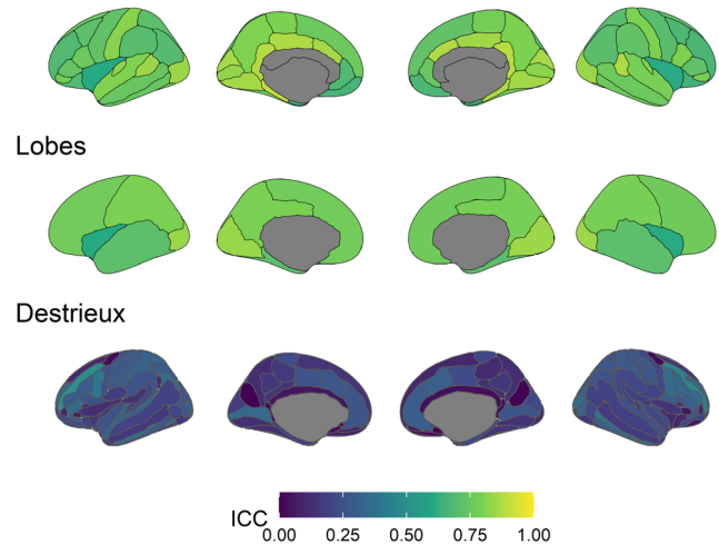
Fig. 11. ICC estimates for cortical thickness for the Desikan-Killiany-Tourville parcellation (top), the combined lobes from the Desikan-Killiany-Tourville parcellation (middle), and the Destrieux parcellation (bottom). Lighter colours indicate higher longitudinal stability.
