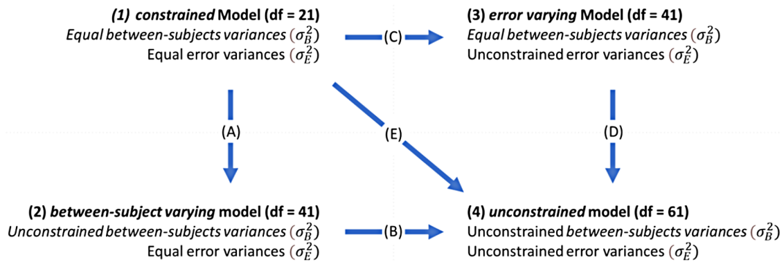
Fig. 6. Representation of multigroup ICED models (numbers 1-4), and model comparisons (arrows A-E). The model descriptions refer to whether the between-subjects variance ( \sigma_B^2 ) and error variance ( \sigma_E^2 ) parameters were allowed to vary across sites (unconstrained) or were set to be equal across sites (equal). The arrows represent the model comparisons ( \Delta CFI) in the direction towards the less constrained model.
