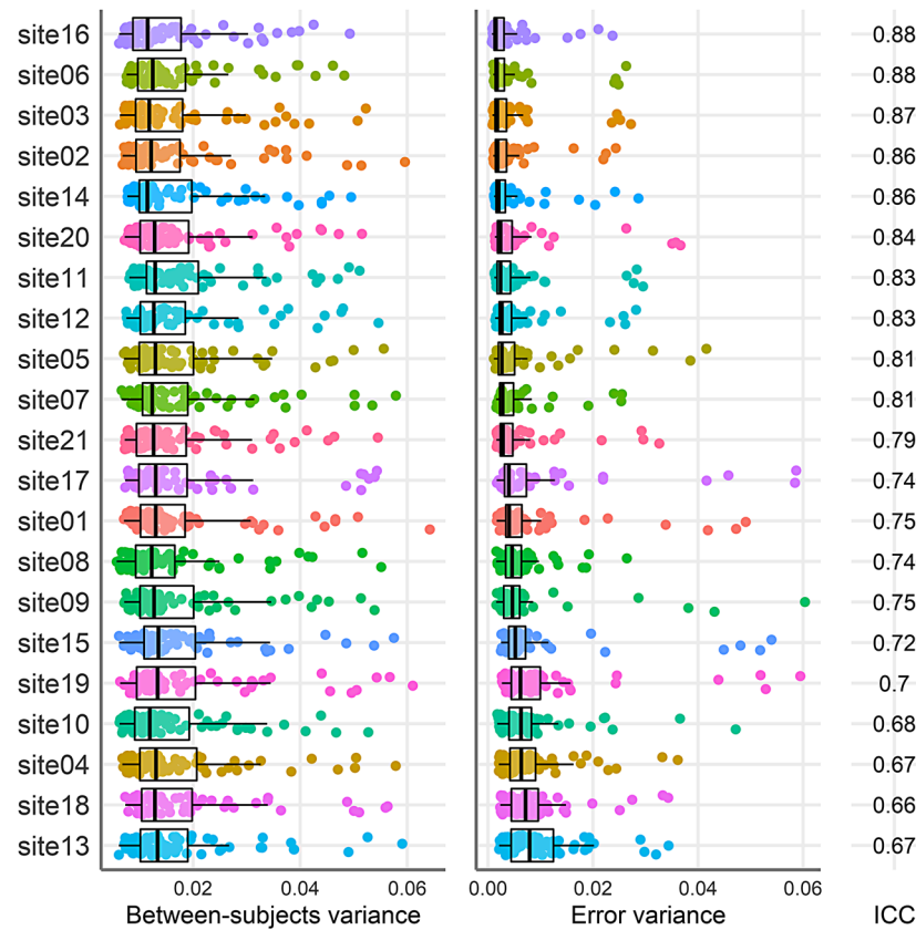
Fig. 5. Between-subjects (left panel), error variance (middle panel) estimates, separately per testing site. Sites are ordered by the median error variance. Each point represents a different brain region, and the site colour maps to Figure 4. Cortical thickness only. The boxplots present the median and the 25 th and 75 th percentiles, the whiskers extend at a maximum to 1.5 times the interquartile range from the box.
