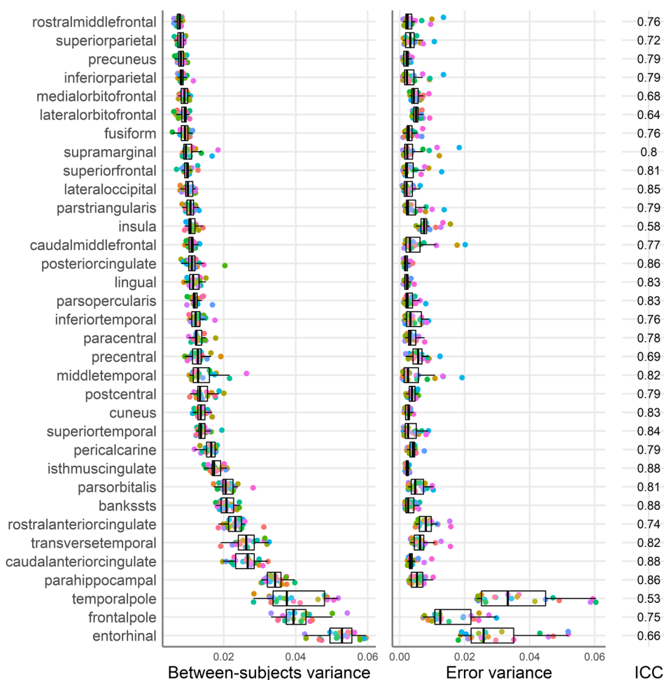
Fig. 4. Between-subjects (left panel), error variance estimates (middle panel), and median ICC (right panel) for each region of interest (y-axis). Regions are ordered by the median between-subjects variance. For clarity we present only the right hemisphere regions. Each point represents a different testing site, and the colour mapping is the same as in Figure 5. The boxplots present the median and the 25 th and 75 th percentiles, the whiskers extend at a maximum to 1.5 times the interquartile range from the box.
