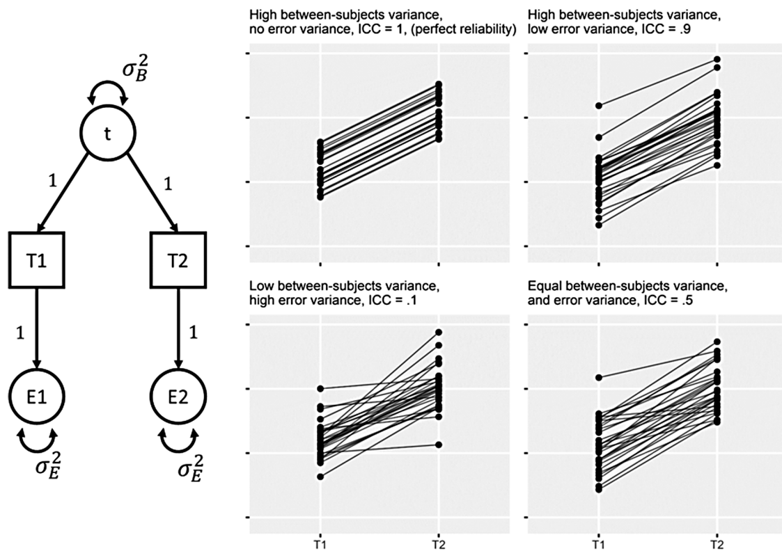
Fig. 1. Left: Path diagram of the two timepoint ICED model used to estimate Between-subjects ( \sigma_B^2 ) and error variance ( \sigma_E^2 ) components. Right: Four plots visualising hypothetical differing levels of between-subjects and error variance, with equal total variance, to depict the relationship between test-retest reliability and rank-ordering individuals.
