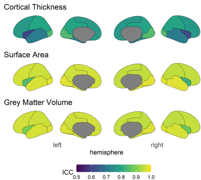
Fig. 9. ICC estimates across structural measures and lobes. Lighter colours indicate higher longitudinal stability.
