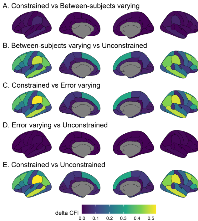
Fig. 7. \Delta CFI for each model comparison (A-E) across regions. Higher values (lighter and more yellow coloured) indicate improved model fit with more free parameters. In comparisons A and D, between-subjects variance is allowed to vary compared to the preceding model. In comparisons B and C, error variance is allowed to vary compared to the preceding model. In panel E, both between-subjects and error variances are allowed to vary compared to the fully constrained model.
