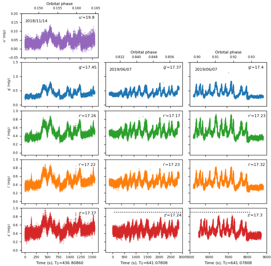
(a) The ULTRACAM light curves
