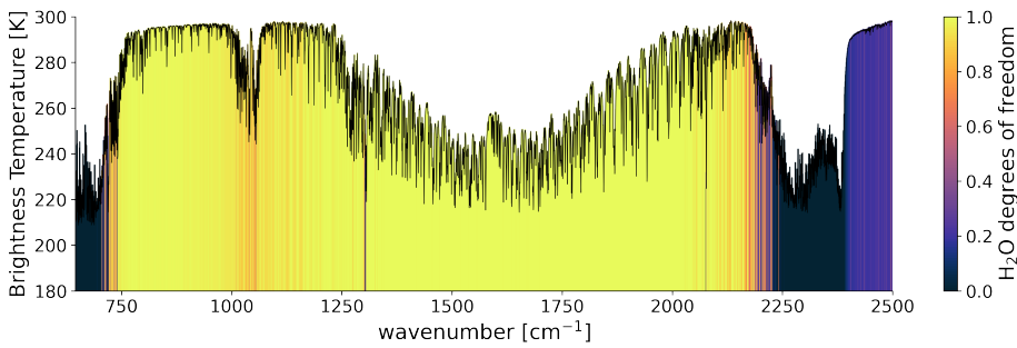
Figure A.1: Forward simulated spectrum in the spectral range of the IASI instrument. Colors denote the water vapor information content of individual channels calculated as the trace of the averaging kernel matrix when only each respective channel is used. Hence, the colored shading does not account for redundancy of information between channels, but simply conveys where water vapor absorption is significant.
