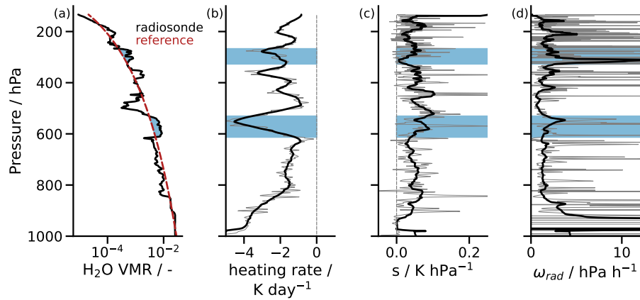
Figure 3.2: GRUAN sounding from 2012-15-02 at 12 UTC of (a) \text{H}_2\text{O} volume mixing ratio (VMR), (b) longwave heating rate, (c) static stability and (d) radiatively driven vertical velocity. The dashed red line in (a) is the reference humidity profile against which EMLs are identified, which are highlighted by blue shaded regions. Thin gray lines in (b), (c) and (d) indicate raw data and thick lines 500 m moving averages to visually remove some strong fluctuations.
