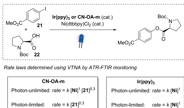
Figure 15. Rate laws of a metallaphotocatalytic C–O arylation obtained using ATR-FTIR monitoring and VTNA using two different photocatalysts under photon-limited and photon-unlimited reaction regimes.
