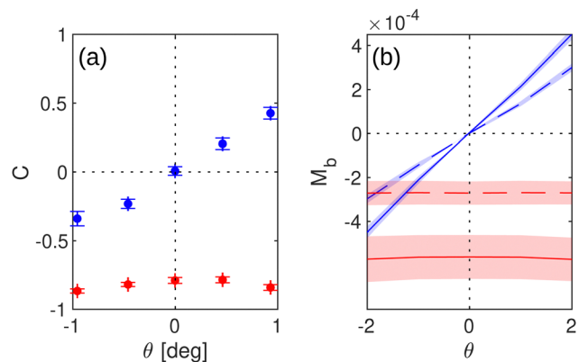
Fig. 6 (a) Cross-correlations vs. theta: blue circles correspond to C_{v_z, \omega}(\theta) , red circles correspond to C_{v_x, \omega}(\theta) . (b) Cross-mobilities M_{b, zy} (blue) and M_{b, xy} (red) vs. theta: solid lines represent simulations with slip BC, while dashed lines the simulations with no-slip BC.
