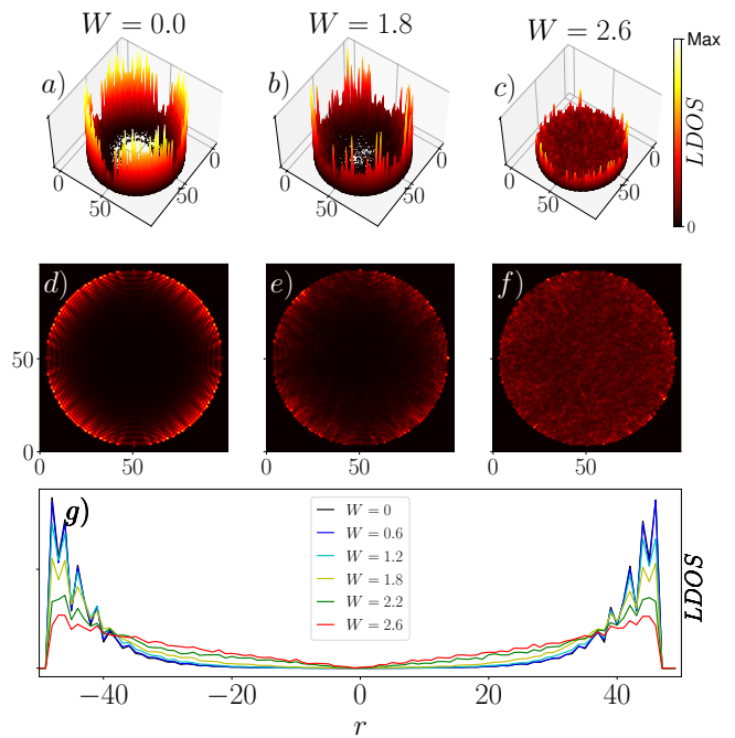
FIG. 7. Local DOS for subgap energies |E| < \Delta_{\text{Topo}}/4 in the topological phase for a finite disc of radius r = 47 . 2D and 3D plots of the local DOS in the clean limit (a,d) and for W = 1.8 (b,e) and W = 2.6 (c,f). (g) Line cuts of the local DOS in same low-energy range through the disc for different disorder strengths W .
