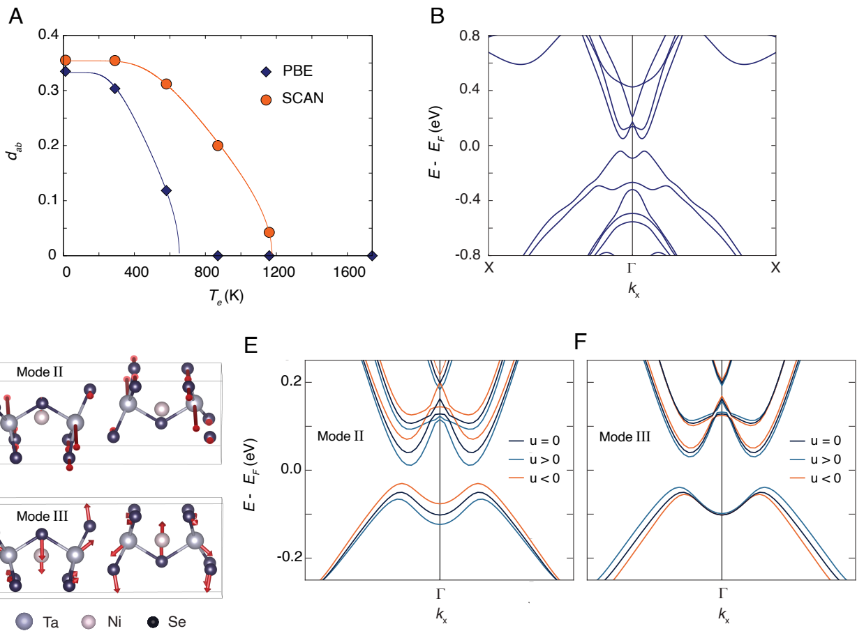
Fig. 4. (A) Distance between the calculated monoclinic structure and the nearest orthorhombic structure, evaluated as a function of T_e . In the computation, we used two different density functionals: PBE (blue symbols) and SCAN (orange symbols). The lines are fits to the standard mean-field behavior, d_{ab}(T_e) = d(0)\sqrt{\tanh(T_c/T_e) - 1} , where T_c = 328 K. (B) Calculated electronic structure of \text{Ta}_2\text{NiSe}_5 in the low-temperature monoclinic unit cell along the X-\Gamma-X momentum direction (parallel to the Ta and Ni chains). The electronic structure is computed using GW calculations. A bandgap opens in the single-particle band structure, and its lower value is close to the \Gamma point of the Brillouin zone ( SI Appendix, section S8 for details). The VB (CB) dispersions acquire an M-like (W-like) shape around \Gamma , consistent with the dispersion found in experiments. (C and D) Calculated eigenvectors of the dynamical matrix of \text{Ta}_2\text{NiSe}_5 corresponding to modes II and III, respectively. Violet atoms refer to Ta, pink atoms to Ni, and blue atoms to Se. The phonon spectrum has been computed using DFT. To enhance the visibility of the atomic motion, the amplitude is scaled by a factor of 8. (E and F) Calculated electronic structure of \text{Ta}_2\text{NiSe}_5 displaced along the eigenvectors of the modes showed in panels C and D. The dark blue lines refer to the electronic structure of the initial (undisplaced, u = 0 ) low-temperature unit cell, whereas the light blue (orange) lines indicate the band structure for positive (negative) displacements. The electronic structures are computed on the GW level of theory.
