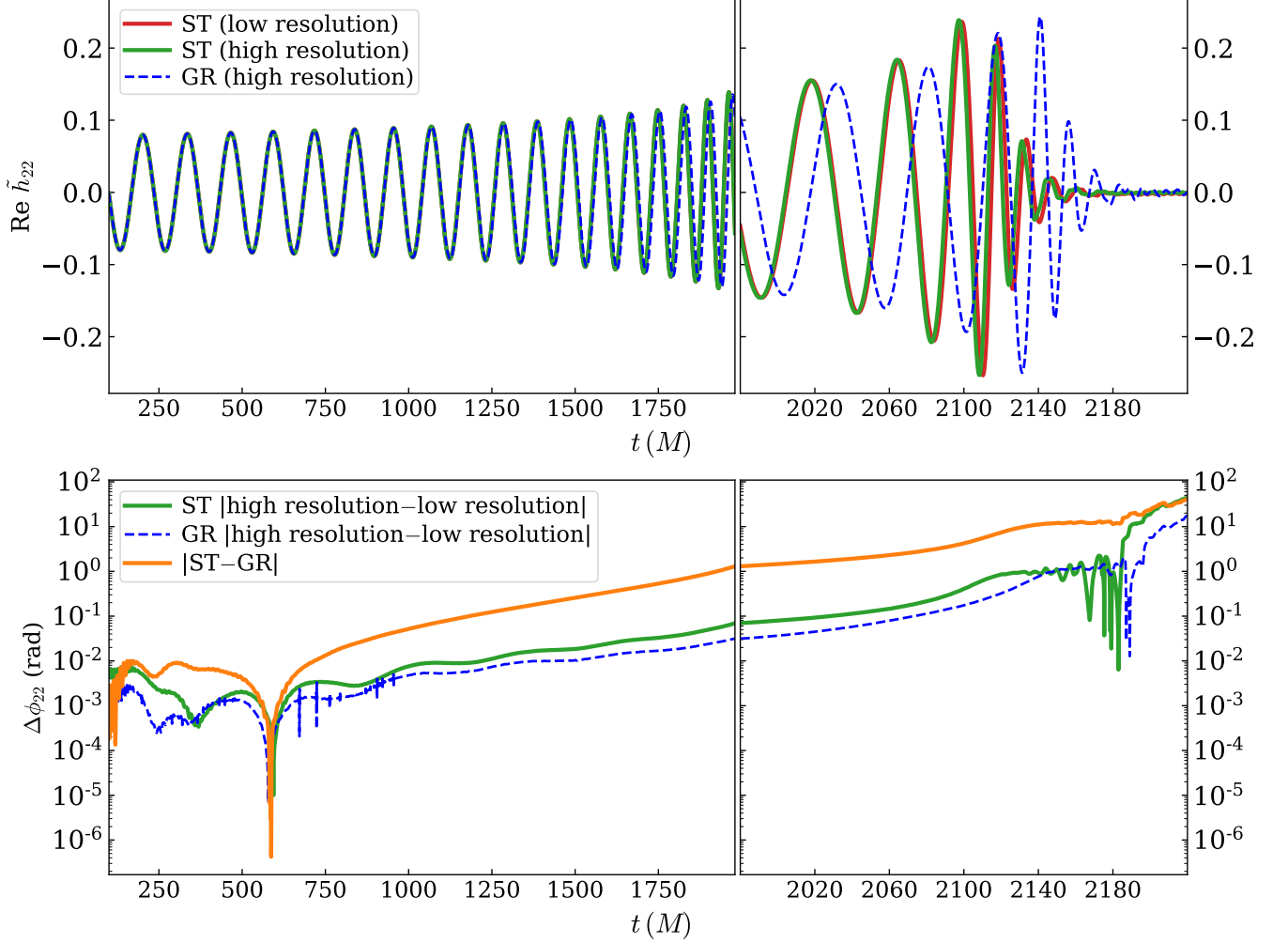
FIG. 9. Upper panel: The ST waveforms with a low (in red) and high (in green) resolution. They are compared to the GR waveform (in blue). Lower panel: the phase difference between the GR and ST waveforms (in orange). For reference, the numerical resolution differences of the GR and the ST waveform are also presented in blue and green, respectively. In addition, we summarize some of the binary parameters in the title.
