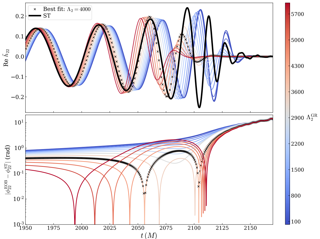
FIG. 12. Comparing the ST waveform (black) with the SEOBv4T model, with a variety of \Lambda_2^{\text{GR}} , ranging from 0 to 6000. The minimum mismatch \mathcal{M} \sim 0.023 happens at \Lambda_2^{\text{GR}} \sim 4000 .
