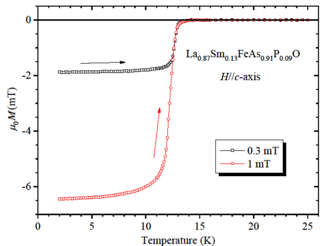
Fig. 3. Temperature-dependent dc magnetization measured in zero-field-cooled (ZFC) mode at 0.3 and 1 mT, with the field applied parallel to the c -axis of a \text{La}_{0.87}\text{Sm}_{0.13}\text{FeAs}_{0.91}\text{P}_{0.09}\text{O} crystal. The sharp superconducting transition at T_c = 13.3 K indicates a good crystal quality, while the strong diamagnetic response well below T_c is consistent with bulk superconductivity.
