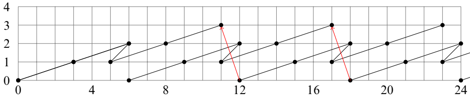
Figure 15: Differentials d_3 .
