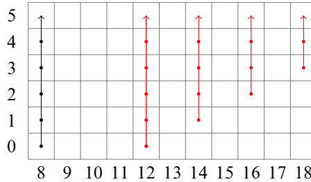
Figure 3: G_2 . The red part is the contribution of \text{Ext}_{\mathcal{A}(0)_*}^{s,t}(\mathbb{F}_2, \mathbb{F}_2) and the black one of \text{Ext}_{\mathcal{A}(1)_*}^{s,t}(\mathbb{H}_*(C_\eta)) .
