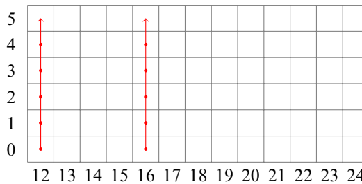
Figure 6: \text{Ext}_{\mathcal{A}(1)_*}^{s,t}(R_3/\Sigma^{18}H_*(C_\eta)) .
