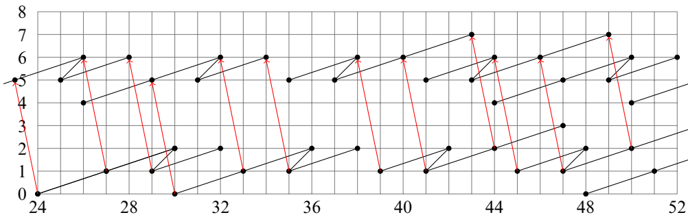
Figure 16: Differentials d_5 .
