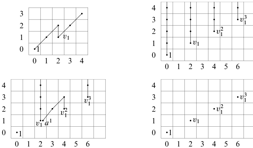
Figure 2: Clockwise from top left: \text{Ext}_{\mathcal{A}(1)_*}^{s,t}(\mathbb{H}_*(V(0))) in the range 0 \leq t - s \leq 4 and \text{Ext}_{\mathcal{A}(1)_*}^{s,t}(\mathbb{H}_*(C_\eta)) , \text{Ext}_{\mathcal{A}(1)_*}^{s,t}(\mathbb{H}_*(S^0 \cup_2 e^1 \cup_\eta e^2)) and \text{Ext}_{\mathcal{A}(1)_*}^{s,t}(\mathbb{H}_*(Y)) in the range 0 \leq t - s \leq 6 .
