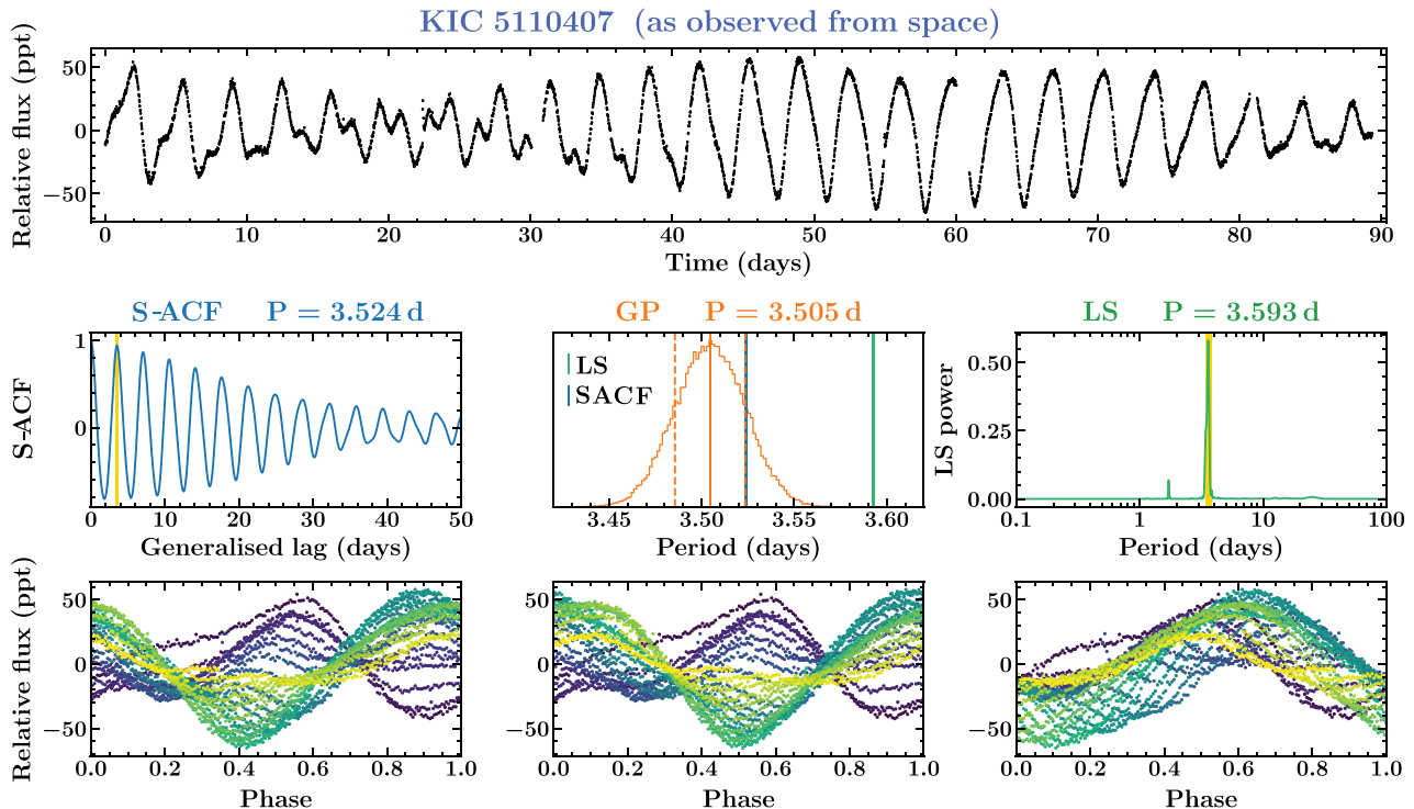
Figure 10. Rotation period estimates for the spotted star KIC 5110407 from S-ACF, GP regression, and LS periodogram. Top panel: the system’s quarter 7 Kepler light curve. Middle left: S-ACF (blue) with the identified period highlighted (yellow). Middle centre: GP posterior period distribution (orange) with the median and 1\sigma uncertainties highlighted (solid and dashed orange lines). For comparison, the S-ACF and LS periods are also shown (blue and green solid lines, respectively). Middle right: LS periodogram (green) with the identified period highlighted (yellow). Bottom row: the Kepler light curve phase-folded on the corresponding method’s period (S-ACF, GP, and LS; left to right) and coloured from the beginning (blue) to the end (yellow) of the observations.
