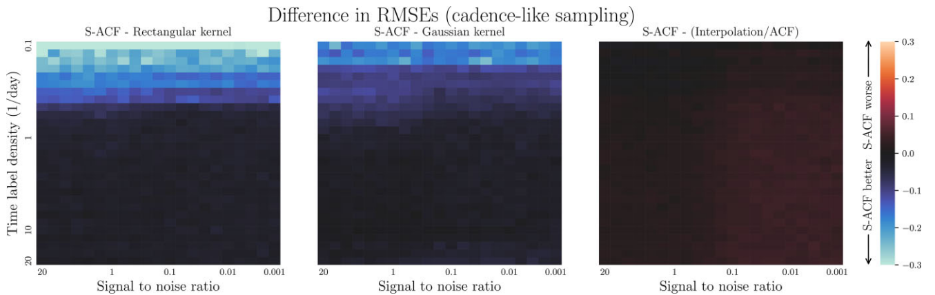
Figure 9. Same as Fig. 8 but for time series with a cadence-like sampling.
