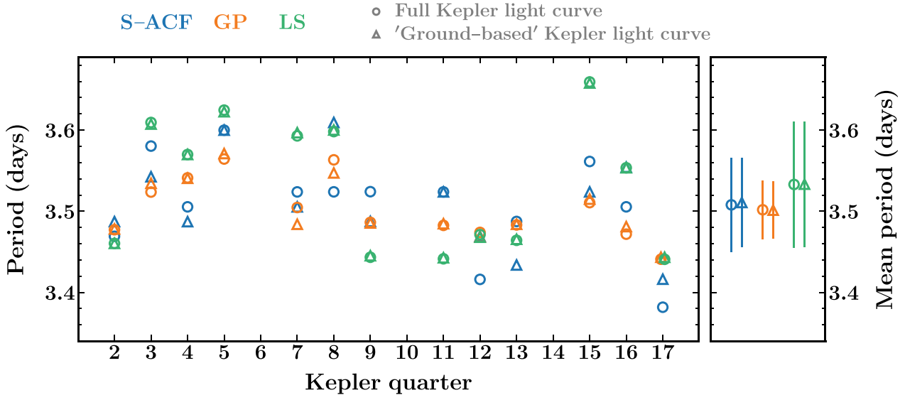
Figure 12. Rotation period estimates for KIC 5110407 from S-ACF (blue), GP (orange), and LS (green) for all quarters with Kepler data. Circles show the period estimates from the full Kepler light curve and triangles from the ‘ground-based’ version of the light curve. The S-ACF periods typically agree better with the GP periods than with LS, especially in cases where there is evolution in the signal shape (e.g. quarters 7 and 15). The right-hand panel shows the mean and standard deviation of the period estimates across all quarters. The mean S-ACF periods from both the full and ‘ground-based’ versions of the light curves agree with each other, and with the values from both the GP and LS methods. The scatter in the S-ACF periods across quarters is smaller than the scatter in LS periods but larger than the scatter in GP periods.
