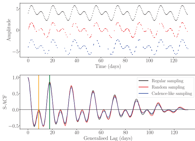
Figure 3. Same as Fig. 2 but for a time series with an underlying process described by the sum of two sine functions with 8.9 and 17.8 d periods. Vertical orange and green lines are plotted at the periods of the signal (8.9 and 17.8 d, respectively) in generalized lag.
