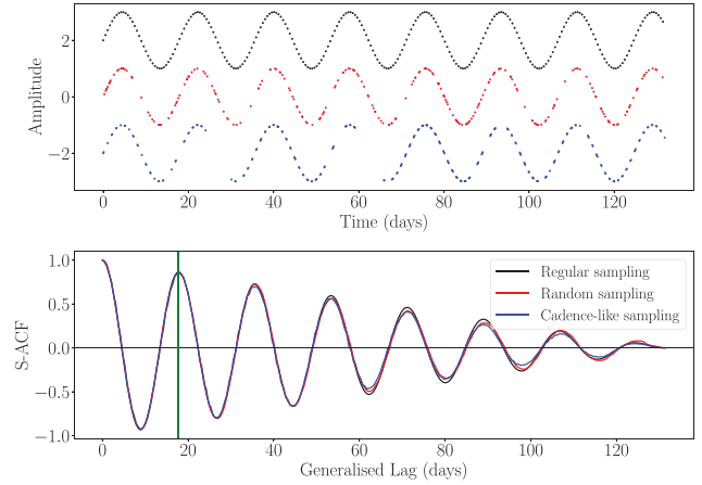
Figure 2. The top panel shows three time series with an underlying sine process (17.8 d period), sampled regularly (black), randomly (red), and with a cadence-like sampling that possesses additional larger gaps (blue). All time label sets have the same cardinality of |T_I| = 250 . The bottom panel shows the S-ACFs of the above time series. A vertical green line is plotted at the period of the signal (17.8 d) in generalized lag.
