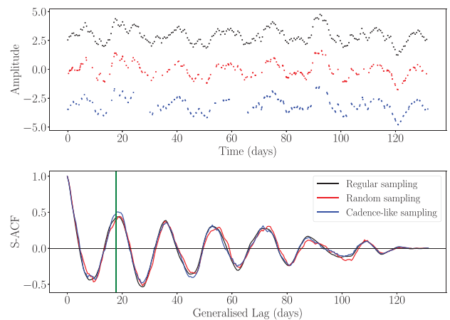
Figure 4. Same as Fig. 2 but for a time series with an underlying process described by the sum of a comparable amplitude sine function and stochastic GP. A vertical green line is plotted at the period of the deterministic component of the signal (17.8 d) in generalized lag.
