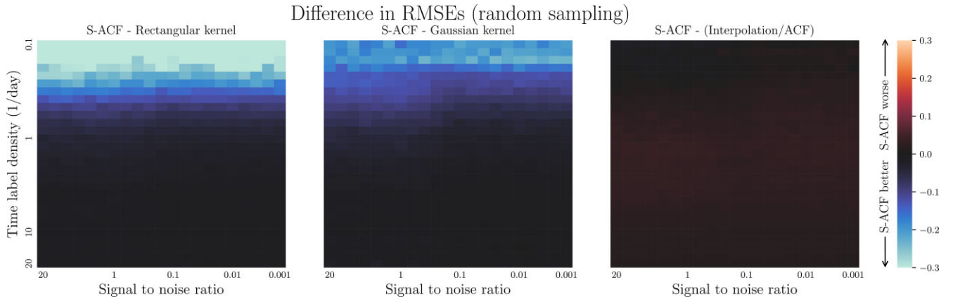
Figure 8. Differences between RMSEs (relative to the standard estimator of the regularly sampled time series) using randomly sampled time series for the S-ACF estimator versus the rectangular kernel estimator (left), the Gaussian kernel estimator (centre), and the standard estimator on the interpolation of the randomly sampled time series (right). These are comparable to the RMSEs of the left-hand panel of Fig. 7. Red indicates a larger RMSE of the S-ACF estimator, blue indicates a larger RMSE of the respective other estimator, and black indicates comparable RMSEs.
