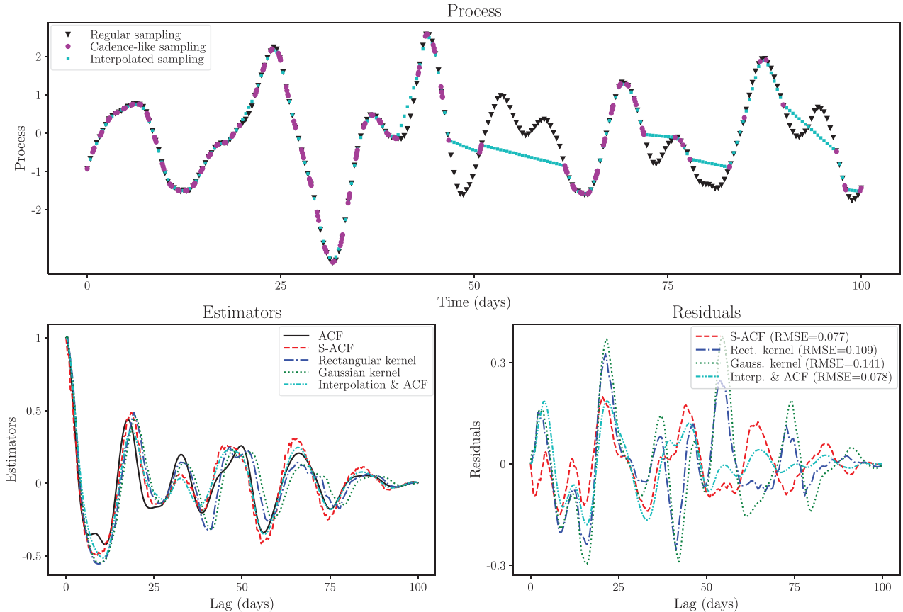
Figure 5. Top: three versions of a process comprising both a periodic component ( P = 17.8 d) and a correlated noise component (characteristic time-scale l = 5 d), which has an average sampling density of 2.5 time labels per day and an S/N of 5.0. The three versions are a regular sampling of the process (black triangles), a cadence-like sampling (magenta circles), and an interpolation of the cadence-like process on to the regular sampling (cyan squares). Bottom left: comparison of the different estimators of the ACF for this process. The standard estimator (black line) is based on the regularly sampled time series. The S-ACF estimator (red dashed), rectangular kernel estimator (blue dash-dotted), and Gaussian kernel estimator (green dotted) are based on the cadence-like sampling of the process. Finally, we use the interpolated regular sampling of the process to again apply the standard estimator (cyan dash-dot-dotted). Bottom right: residuals of the different estimators (S-ACF, rectangular and Gaussian kernels, and interpolation) relative to the standard estimator (i.e. the ACF). RMSEs are indicated in the legend.
