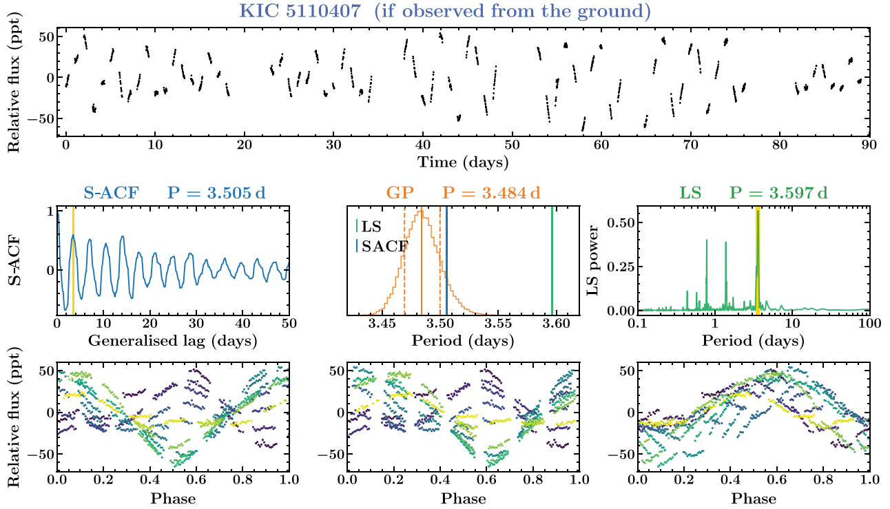
Figure 11. Same as Fig. 10 but simulating KIC 5110407 being observed from the ground (i.e. observations during night-time only with additional gaps from bad weather).
