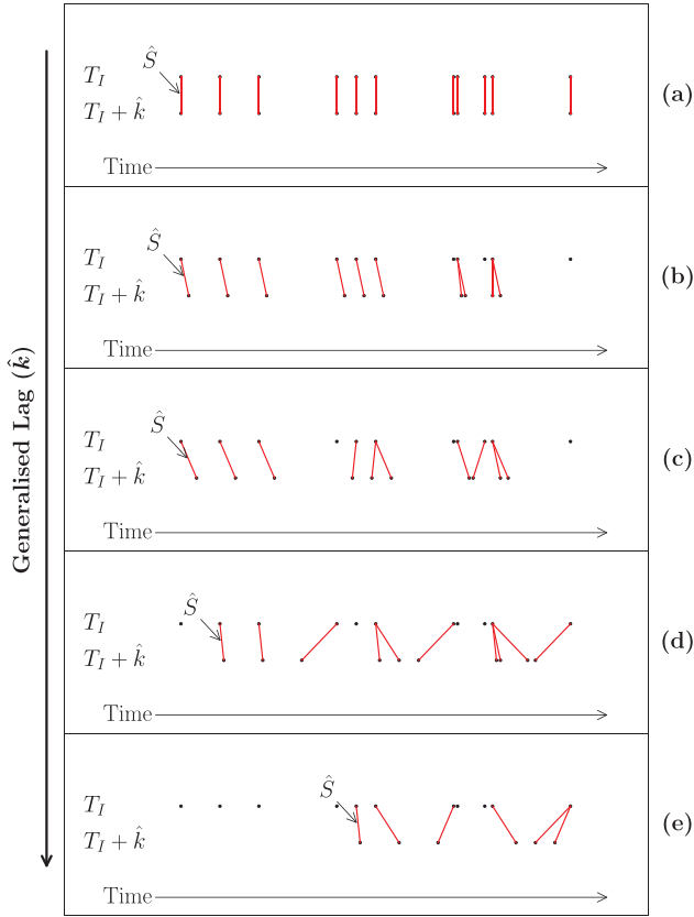
Figure 1. Each graphic (a)–(e) shows a set of time labels on the real axis and below them the same set of time labels shifted by a real generalized lag \hat{k} . The red lines indicate how the selection function \hat{S} matches the shifted time labels to the original set of time labels above by choosing the closest time label from the set of time labels T_I . The generalized lag increases from panel (a) to (e), which corresponds to the lower set of labels ‘shifting’ to the right. A supplementary animated version of this figure is available on the journal website.
