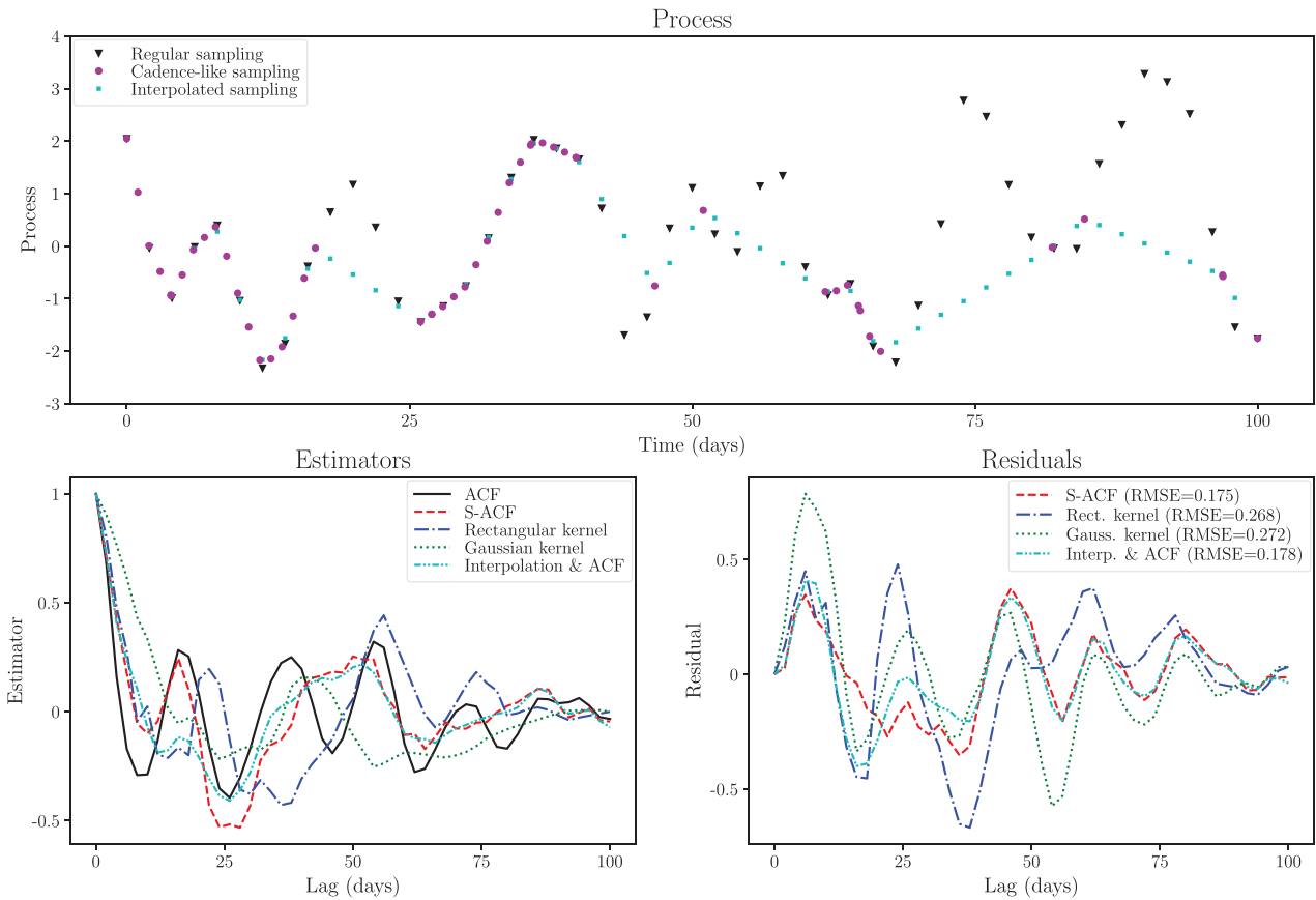
Figure 6. Same as Fig. 5 for a process with a periodic component ( P = 17.8 d) and a correlated noise component (characteristic time-scale l = 15 d), an average sampling density of 0.5 time labels per day, and an S/N of 0.1.
