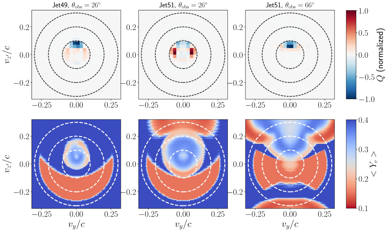
Figure 6. Q maps (top) versus Y_e maps (bottom) for three cases from Fig. 4 showing non-zero polarization levels around 2 d after the merger and at \sim 7000 \text{ \AA} : the Jet49 model viewed from 26^\circ with q < 0 (left), the Jet51 model viewed from 26^\circ with q > 0 (middle), and the Jet51 viewed from 66^\circ with q < 0 (right). All maps are calculated by rotating the xyz Cartesian grid about the y -axis and so that x' corresponds to the line of sight to the given observer, i.e. x' = x \cos(\pi/2 - \theta_{\text{obs}}) + z \sin(\pi/2 - \theta_{\text{obs}}) , y' = y , and z' = -x \sin(\pi/2 - \theta_{\text{obs}}) + z \cos(\pi/2 - \theta_{\text{obs}}) . The Q maps are computed by integrating all the contributions along the line of sight and are normalized to the maximum value across the three cases. The Y_e maps are computed by averaging the Y_e values from 0.075 to 0.15c along the line of sight and on the approaching side of the ejecta. Dashed white circles mark velocities of 0.1, 0.2, and 0.3c as in Fig. 1.
