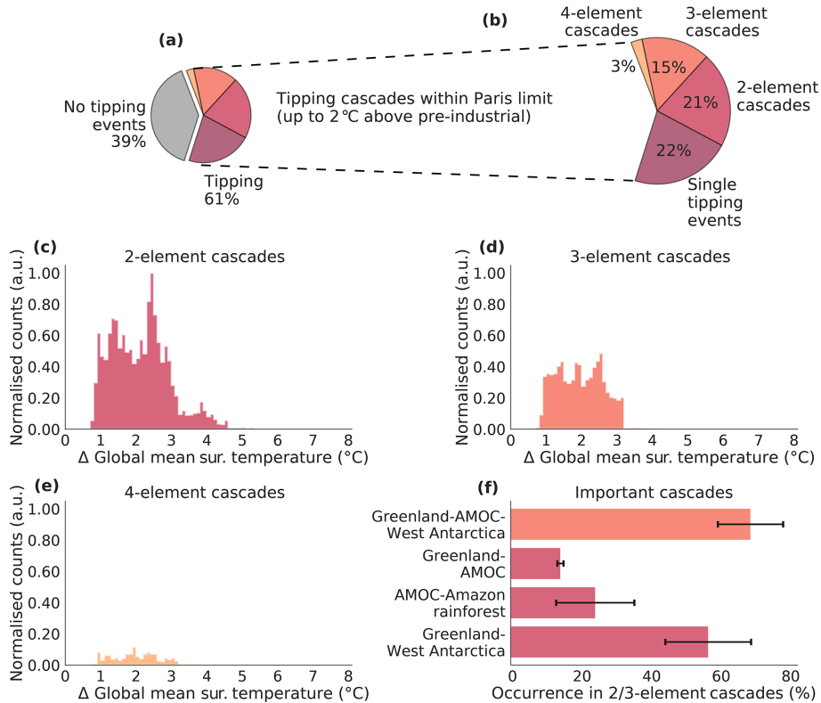
Figure 5. Tipping cascades for all interaction strengths between 0.0 and 1.0. (a, b) For global warming up to 2.0^{\circ}\text{C} above pre-industrial levels, the coloured shading illustrates the fraction of model representations in the Monte Carlo ensemble without tipping events (grey), with a single tipping event (purple), and with cascades including two (red), three (dark orange) or four (light orange) elements. (c–e) Occurrence of tipping cascades with two, three or four elements as a function of global mean surface temperature increase. The counts are normalised to the highest value of the most frequent tipping cascade (in cascades with two elements). (f) Dominant cascades with two and three elements for temperature increases from 0 to 8^{\circ}\text{C} above pre-industrial. Other cascades are not shown, as their relative occurrence is comparatively much smaller. The standard deviation represents the difference between the possible ensemble realisations of the interaction network (see Sect. 2.3). Hence, it tends to be larger for cascades where unclear interaction links are involved, e.g. for the AMOC–Amazon rainforest cascade (compare Fig. 1 and Table 2).
