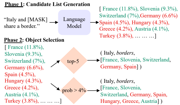
Figure 1: Probing LMs to extract objects for multi-valued relations.
