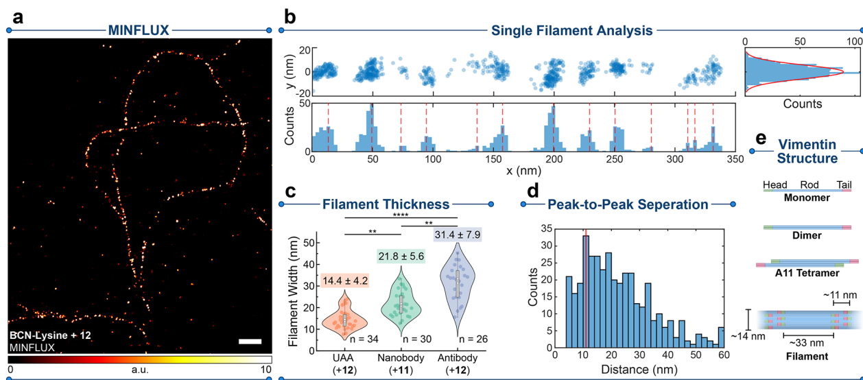
Figure 6. MINFLUX characterization of linkage-error-free labeling. (a) MINFLUX image of vimentin filaments in COS-7 cells incorporating endo BCN- L -lysine as described in Figure 3d and labeled with compound 12. (b) Single filament analysis of the linearized filament marked in panel a; distributions of localizations along the filament length ( x ) and width ( y ) were used to determine peak-to-peak separation of localization domains and the fwhm of the filament segment, respectively. (c) Distribution of filament thicknesses of vimentin segments labeled with different strategies, including UAAs + compound 12, anti-GFP nanobodies + compound 11, and indirect immunofluorescence + compound 12 in transfected COS-7 cells (as described above). The distribution mean \pm SDs are given above the violin plots, and n designates the number of analyzed filament segments. **P < 0.01 ; ****P < 0.0001 using the Kruskal–Wallis and the Dunn method for posthoc correction for multiple comparisons. (d) Peak-to-peak separations of localization domains in vimentin filaments labeled with UAAs. (e) Structure of the vimentin according to recent literature with our obtained values shown. 56 Scale bar: 200 nm.
