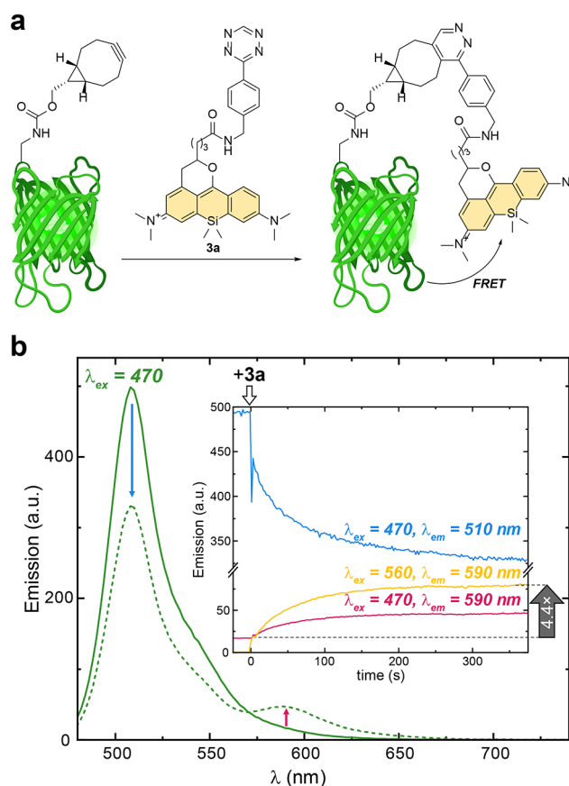
Figure 4. Demonstration of FRET in GFP labeled with a PaX-Tz fluorophore. (a) Schematic representation of GFP-PaX dyad. GFP protein (1.1 eq.; for plasmid details, see the Supporting Information) containing endo BCN- L -lysine 42–46 was reacted with 3a in PBS at pH 7.4. (b) Fluorescence spectra of GFP before (solid line) and after (dashed line) reaction with 3a. Inset: Temporal evolution of the fluorescence signal upon addition of 3a, indicative of FRET from GFP to compound 3a upon SPIEDAC reaction.
