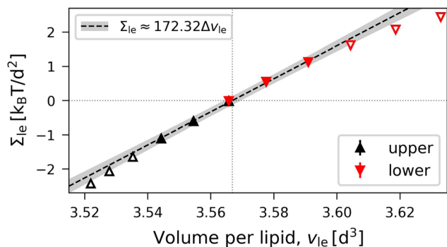
Fig. 7 OLT deformations of planar bilayer assembled from N_{\text{il}} + N_{\text{ul}} = 1682 lipids. The midplanes of the asymmetric OLT states are computed via the VORON protocol: Leaflet tensions \Sigma_{\text{ul}} and \Sigma_{\text{il}} as functions of the volume per lipid, v_{\text{le}} . The dotted vertical line is located at the optimal lipid volume v = v^0 = 3.566d^3 . Filled data symbols represent those v -values that belong to the linear regime and fulfill the linearity condition |\Delta v| < B_{\text{OLT}}/(10B') . The linear fit to these filled data is displayed by the dashed line, the grey shaded band represents the 95% prediction band. The numerical values of the data are displayed in Table S3 (ESI†).
